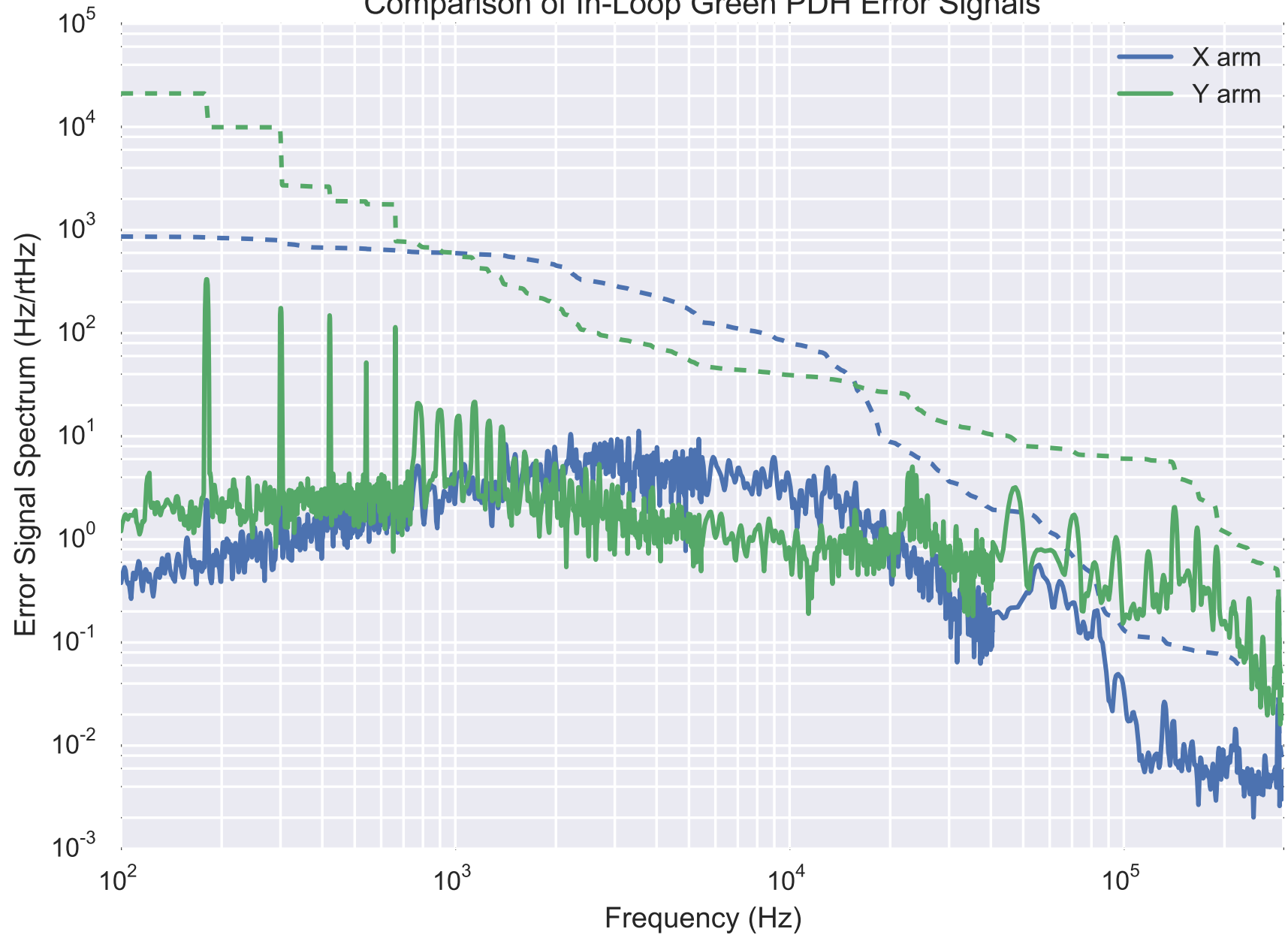
Comparison of In-Loop Green PDH Error Signals
