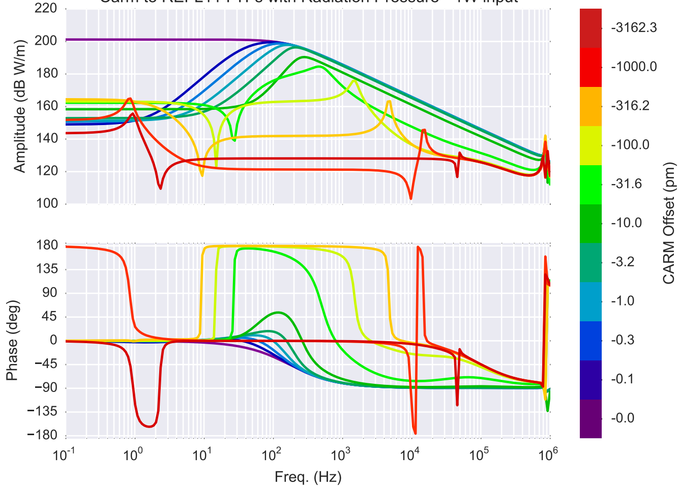
Carm to REFL11 I TFs with Radiation Pressure - 1W input
