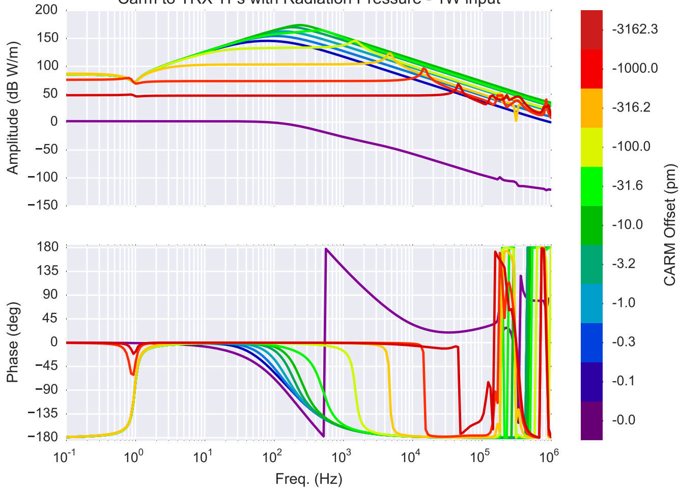
Carm to TRX TFs with Radiation Pressure - 1W input
