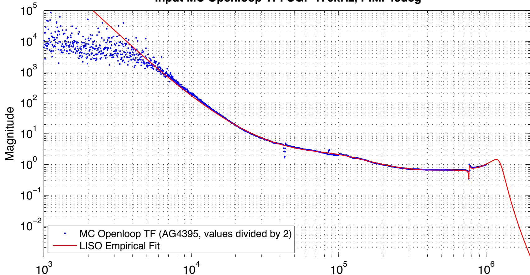
Input MC Openloop TF: UGF 176kHz, P.M. 48deg
