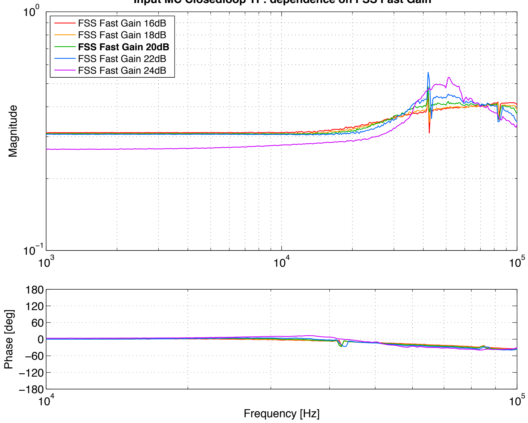
Input MC Closedloop TF: dependence on FSS Fast Gain
