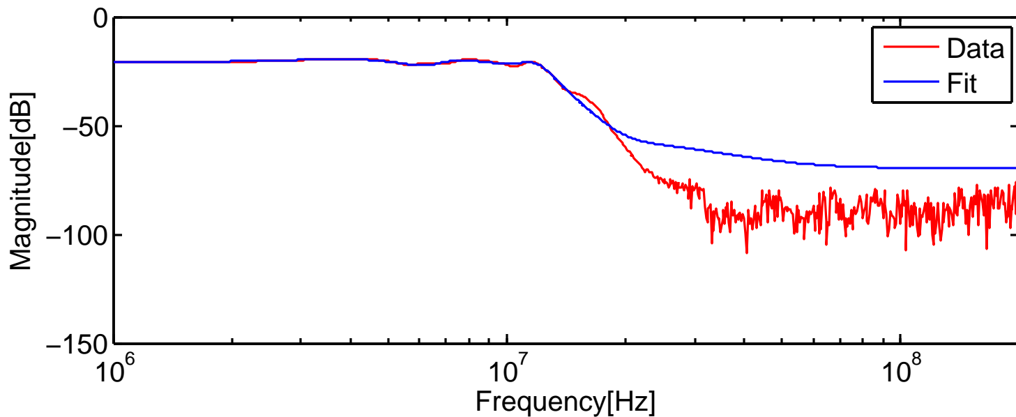
REFL11 Demodulator
