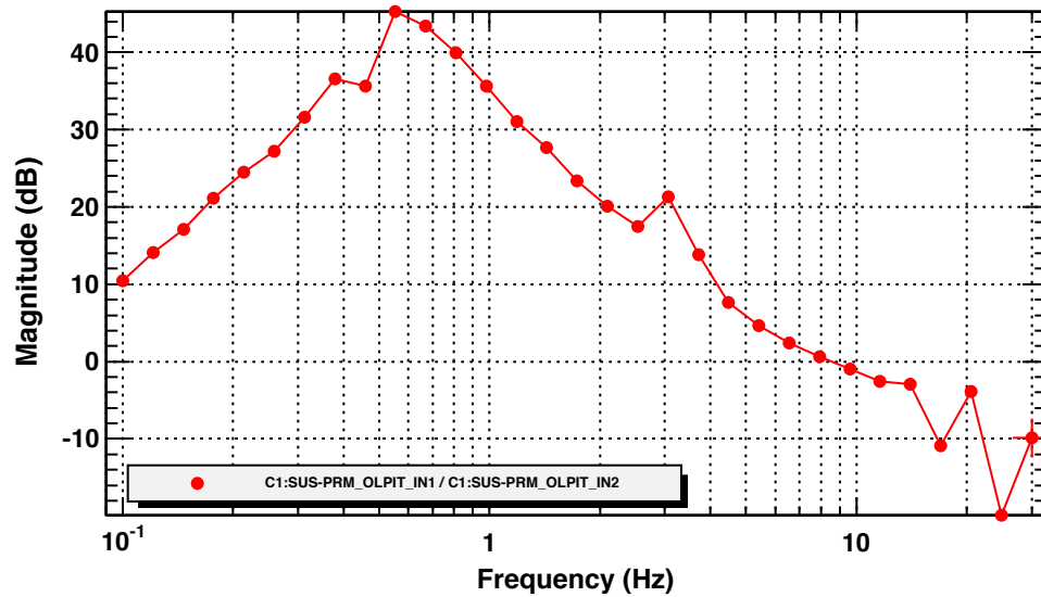
Open Loop Gain
