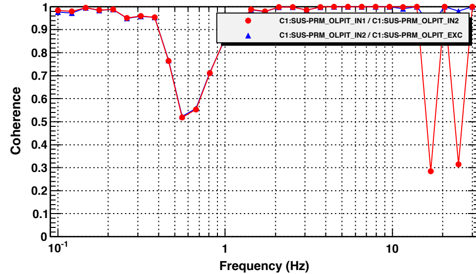
Coherence function
