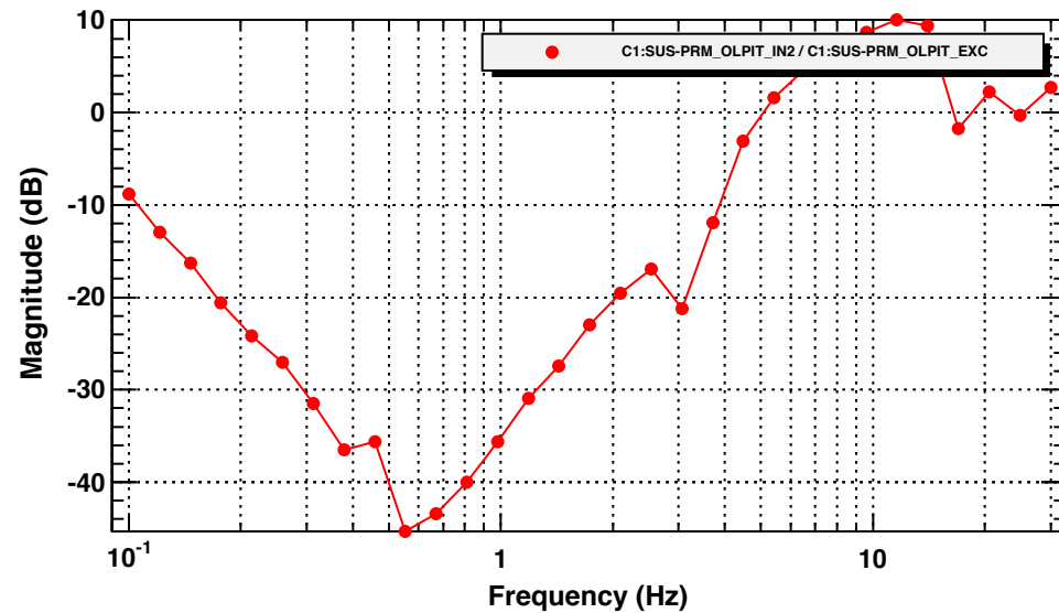
Closed Loop Gain
