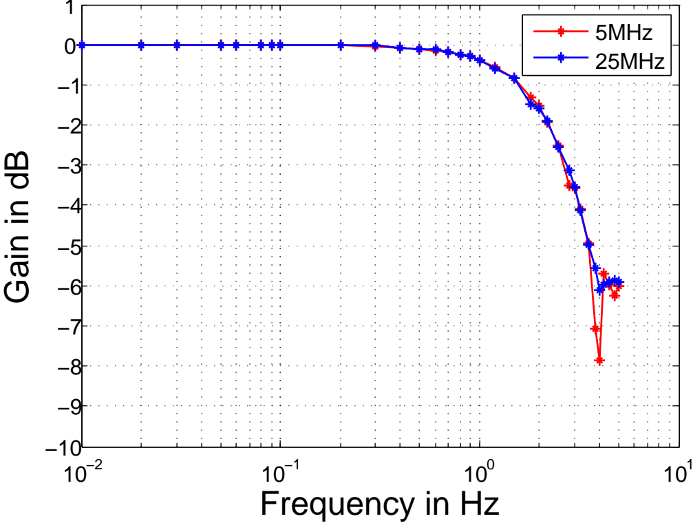
Gain vs Frequency Plot
