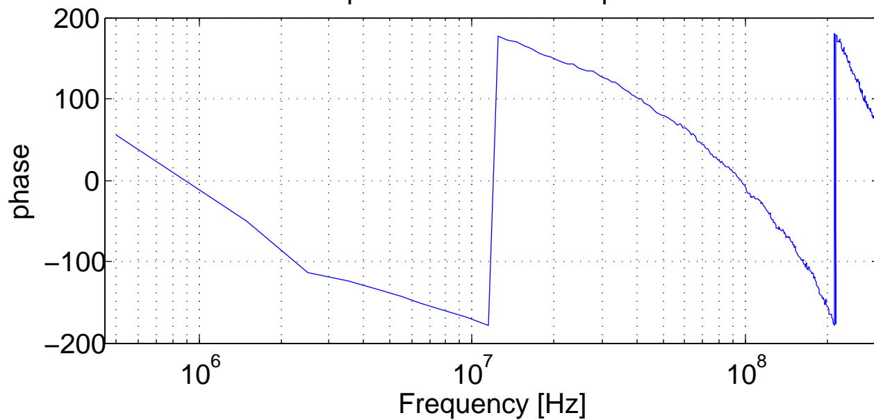
Transimpedance Phase for spare BBPD
