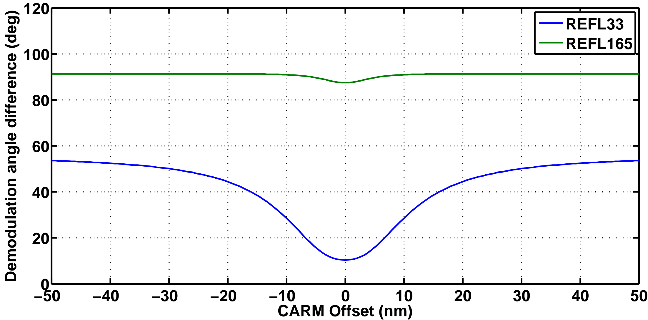
Difference between MICH and PRCL demod angles in 3F signals
