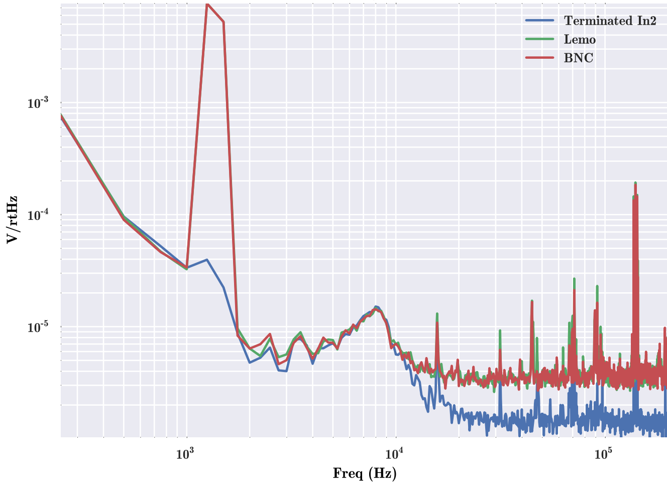
BNC vs. LEMO cable for AO signal - Measured at MC OUT2
