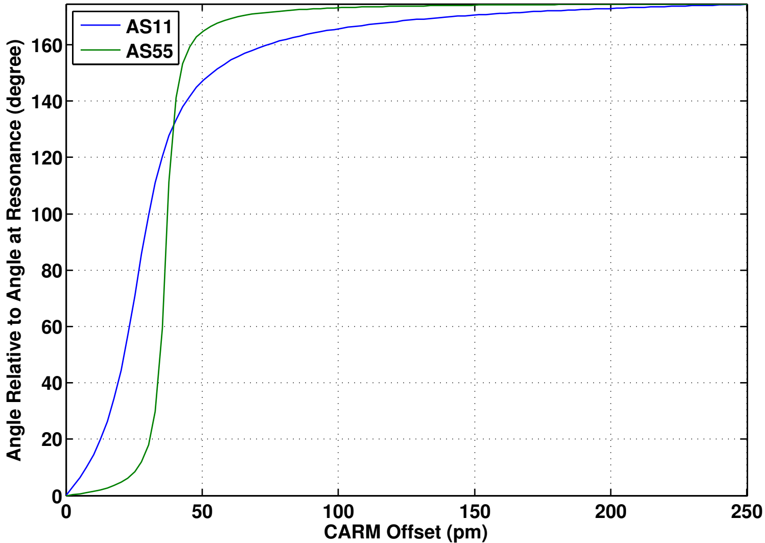
AS DARM demodulation angle with CARM offset
