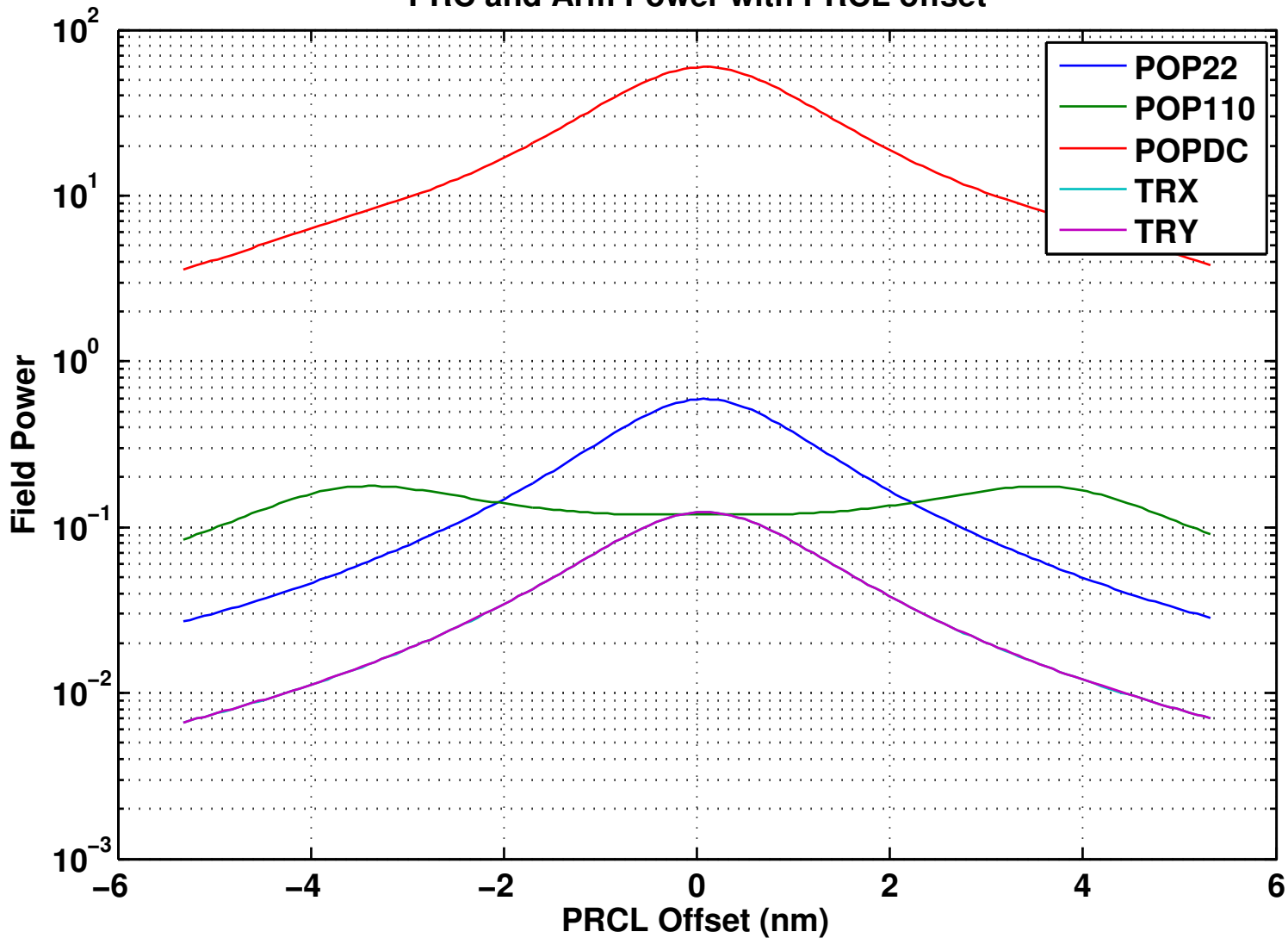
PRC and Arm Power with PRCL offset
