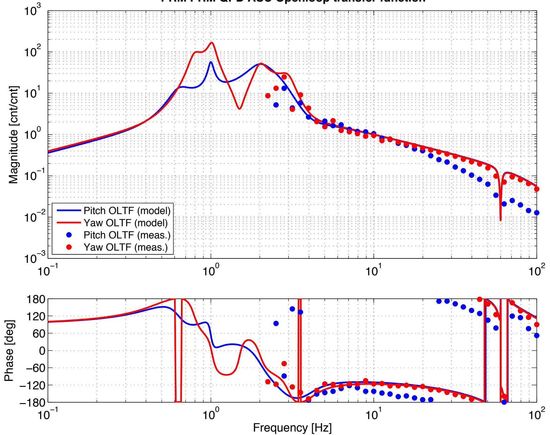
PRM PRM QPD ASC Openloop transfer function
