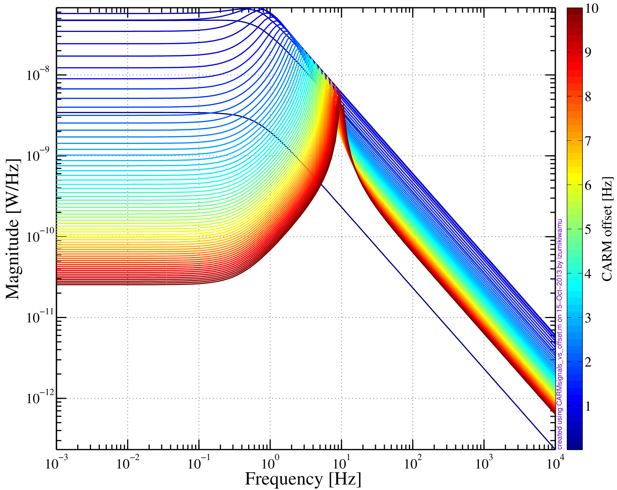
CARM optical gain at REFL DC with various CARM offsets
