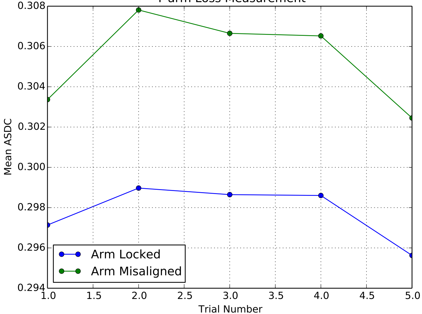
Y-arm Loss Measurement
