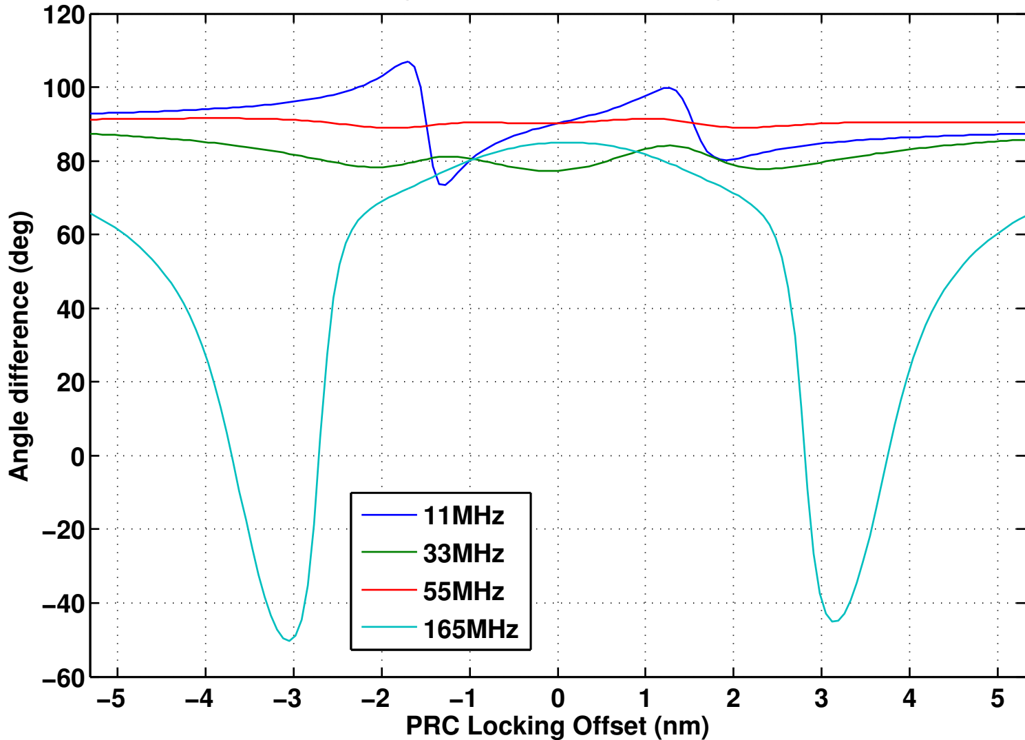
MICH and PRCL Angle in REFL PDs – Locking Offset (Full Scale)
