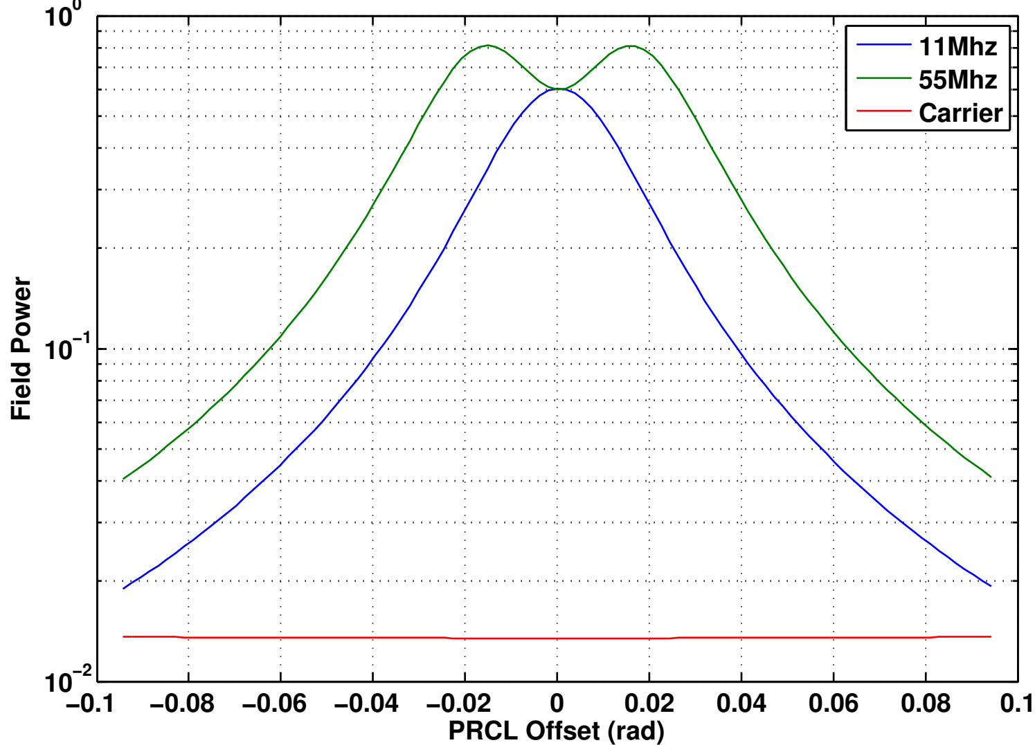
PRC Power with PRCL offset
