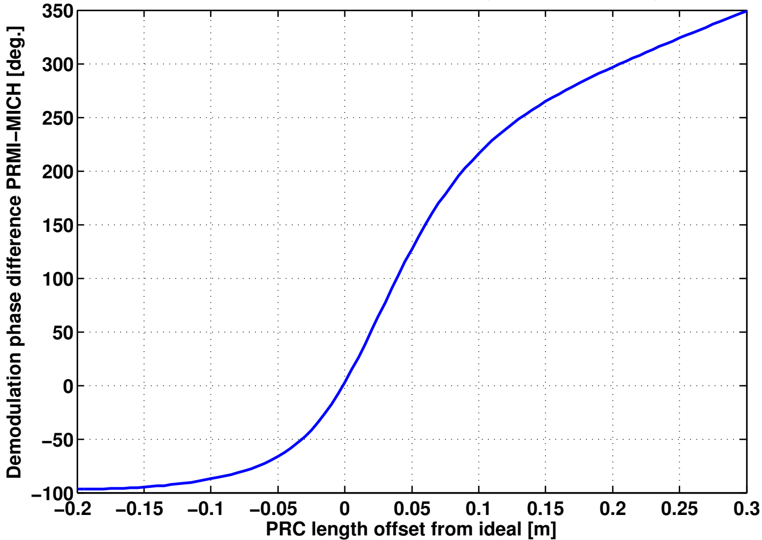
Difference in Demodulation Phase Angles with PRC Length
