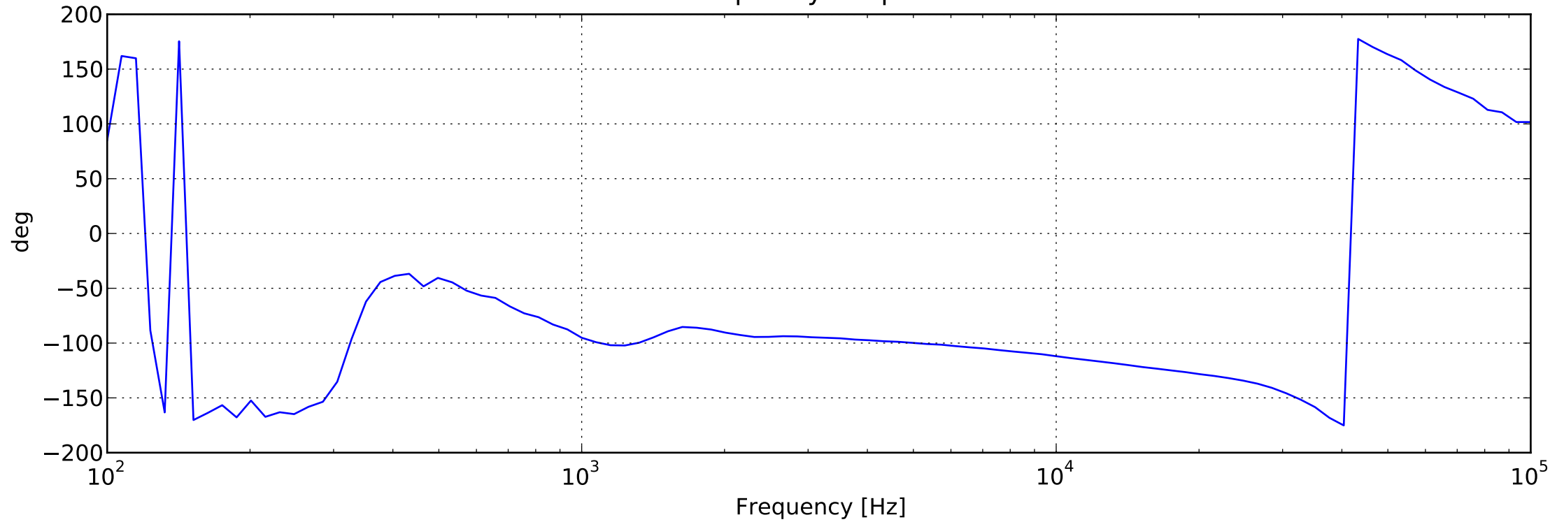
Frequency Response
