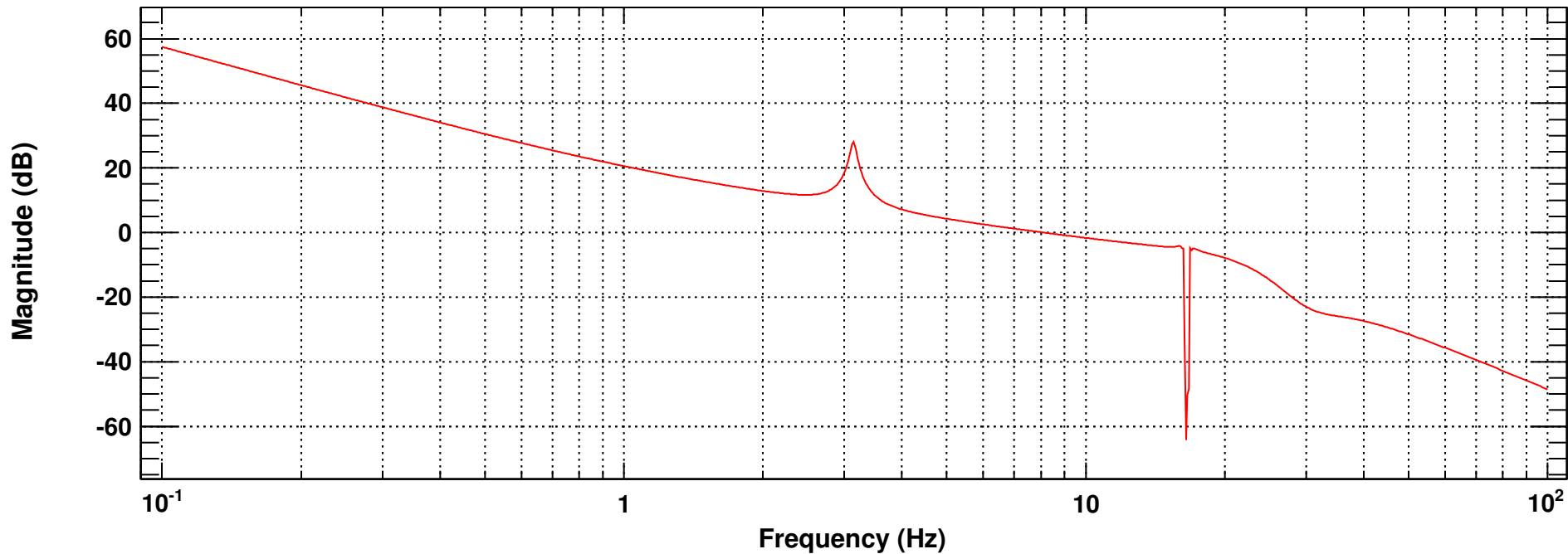
Transfer function
