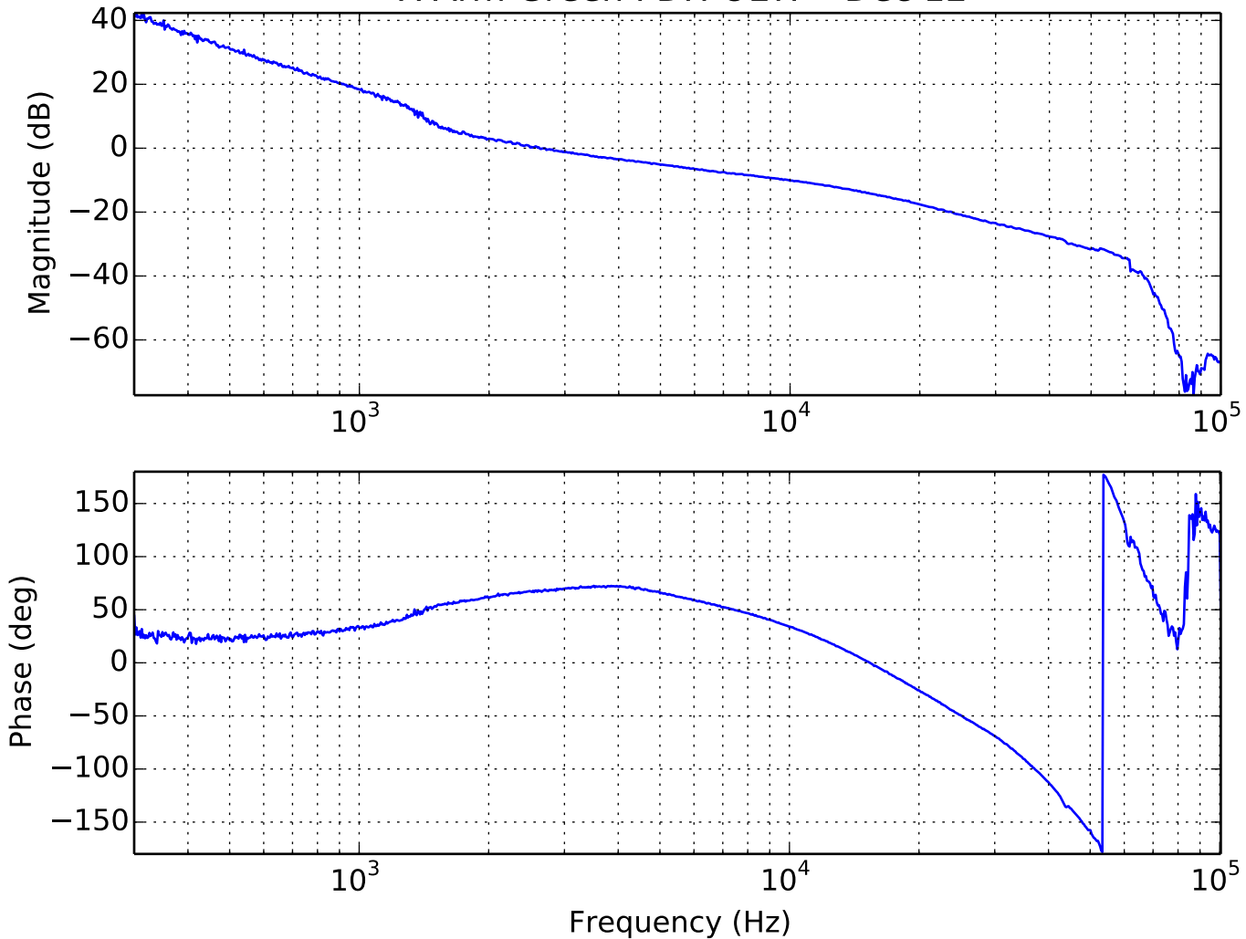
X Arm Green PDH OLTF - Dec 12
