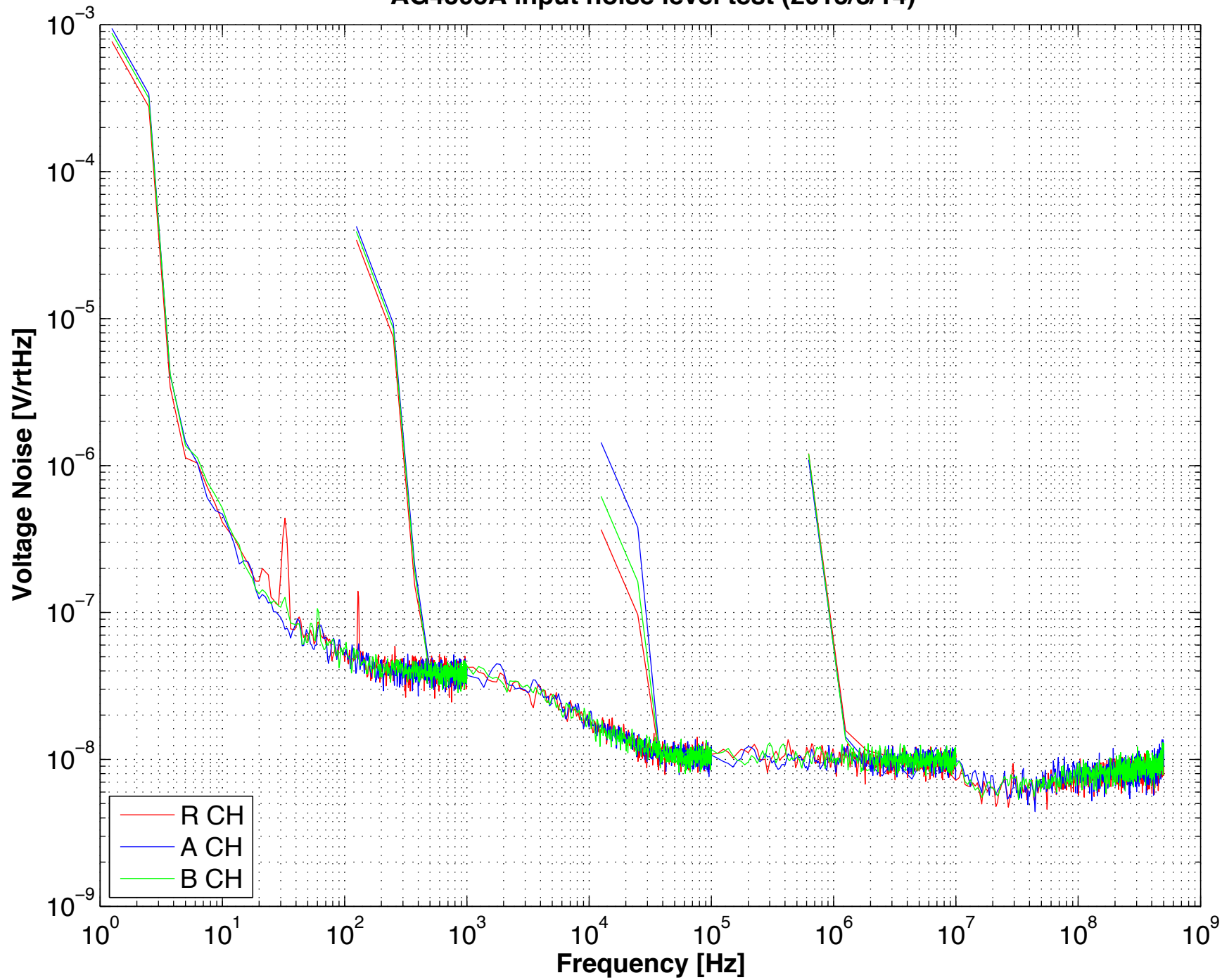
AG4395A input noise level test (2013/8/14)
