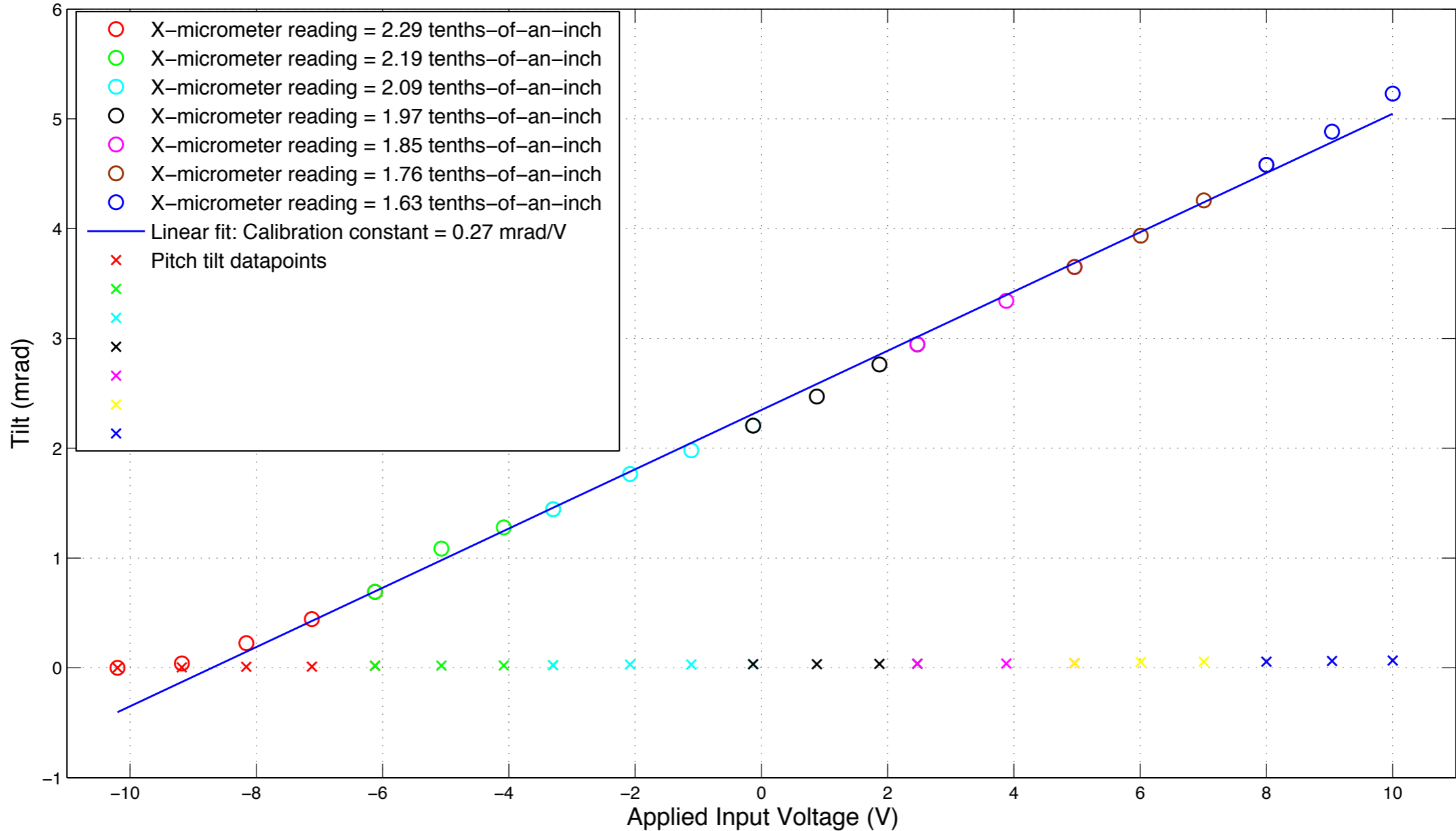
Mirror #2 PZT Calibration – Input to Piezo Yaw (CH1)
