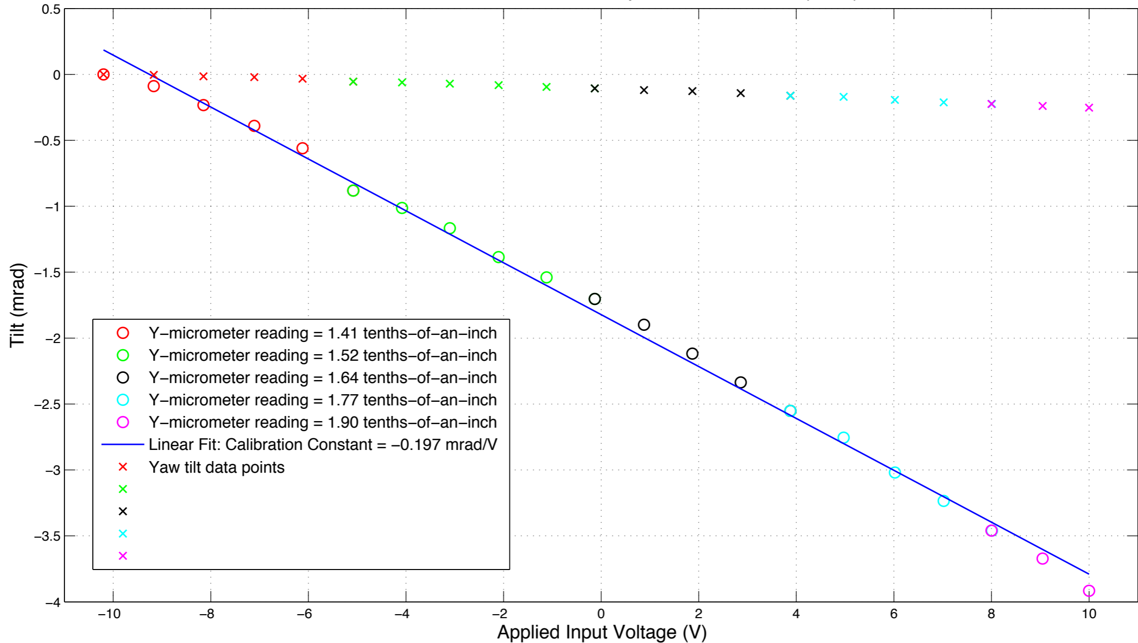
Mirror #2 PZT Calibration – Input to Piezo Pitch (CH2)
