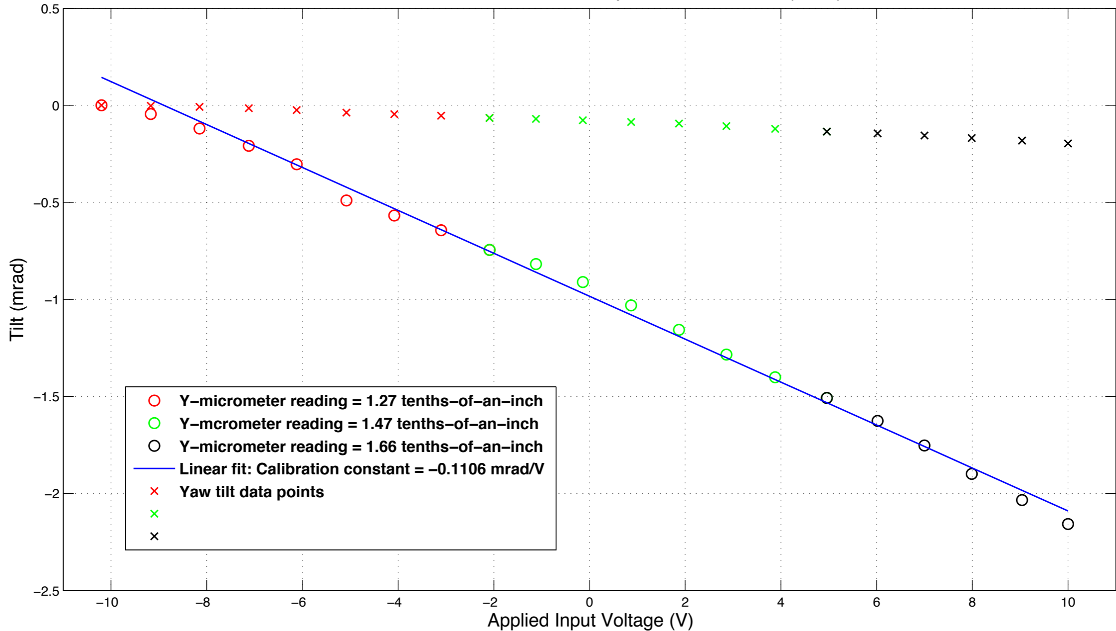
Mirror #1 PZT Calibration – Input to Piezo Pitch (CH2)
