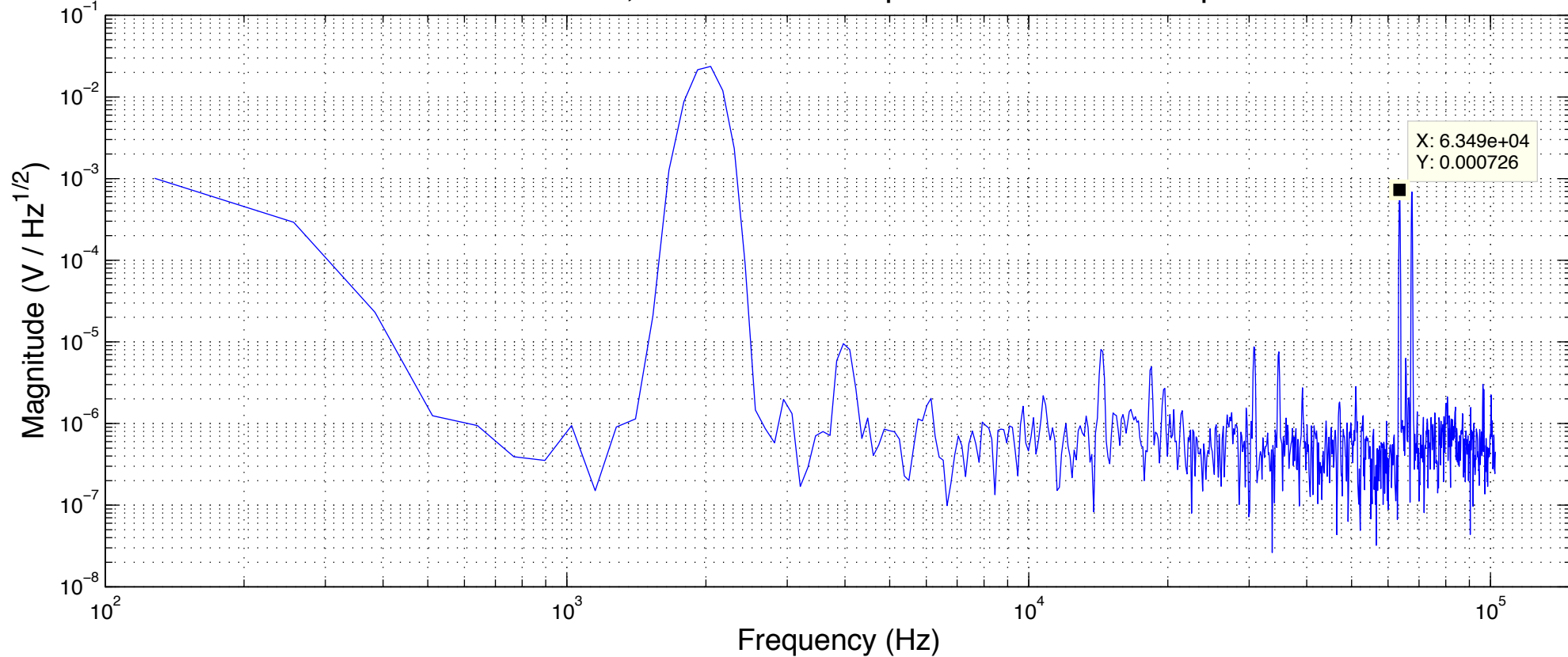
DAC at 1Y4– PSD with 2kHz, 1000 counts amplitude sine wave output from Channel 9
