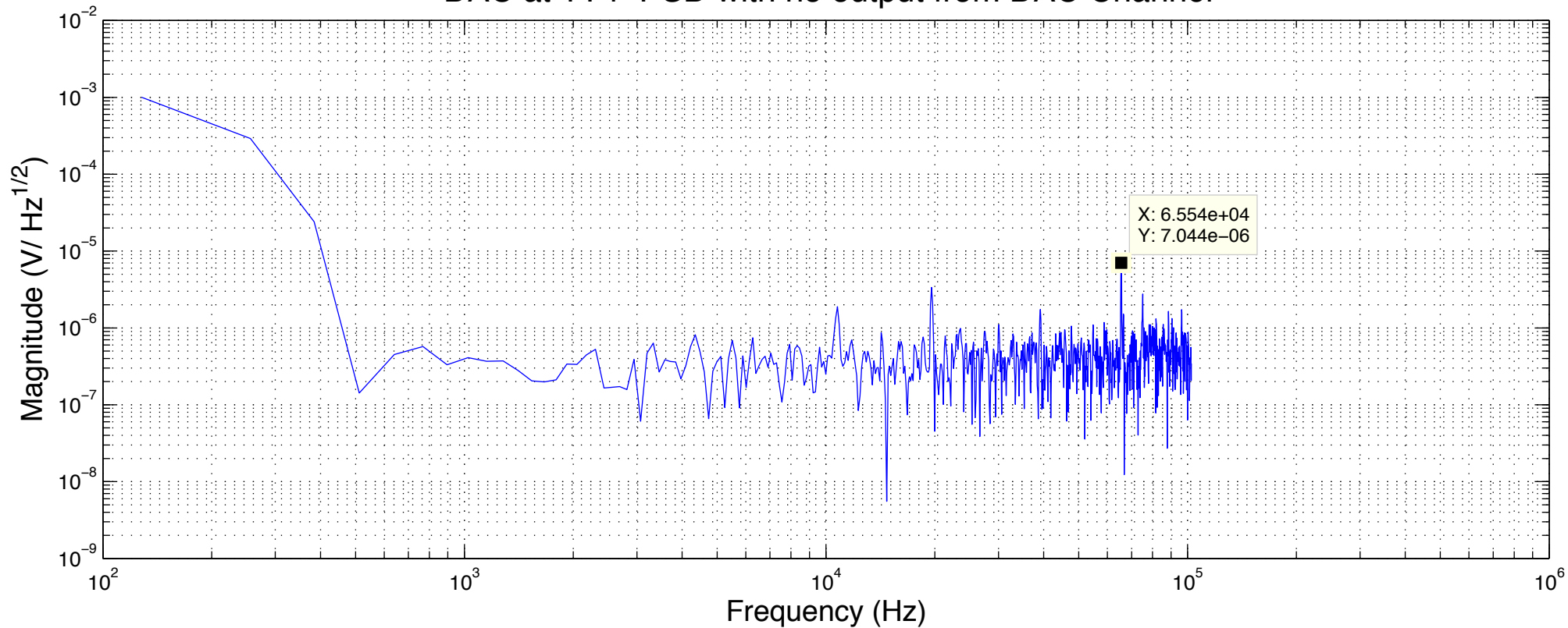
DAC at 1Y4-PSD with no output from DAC Channel
