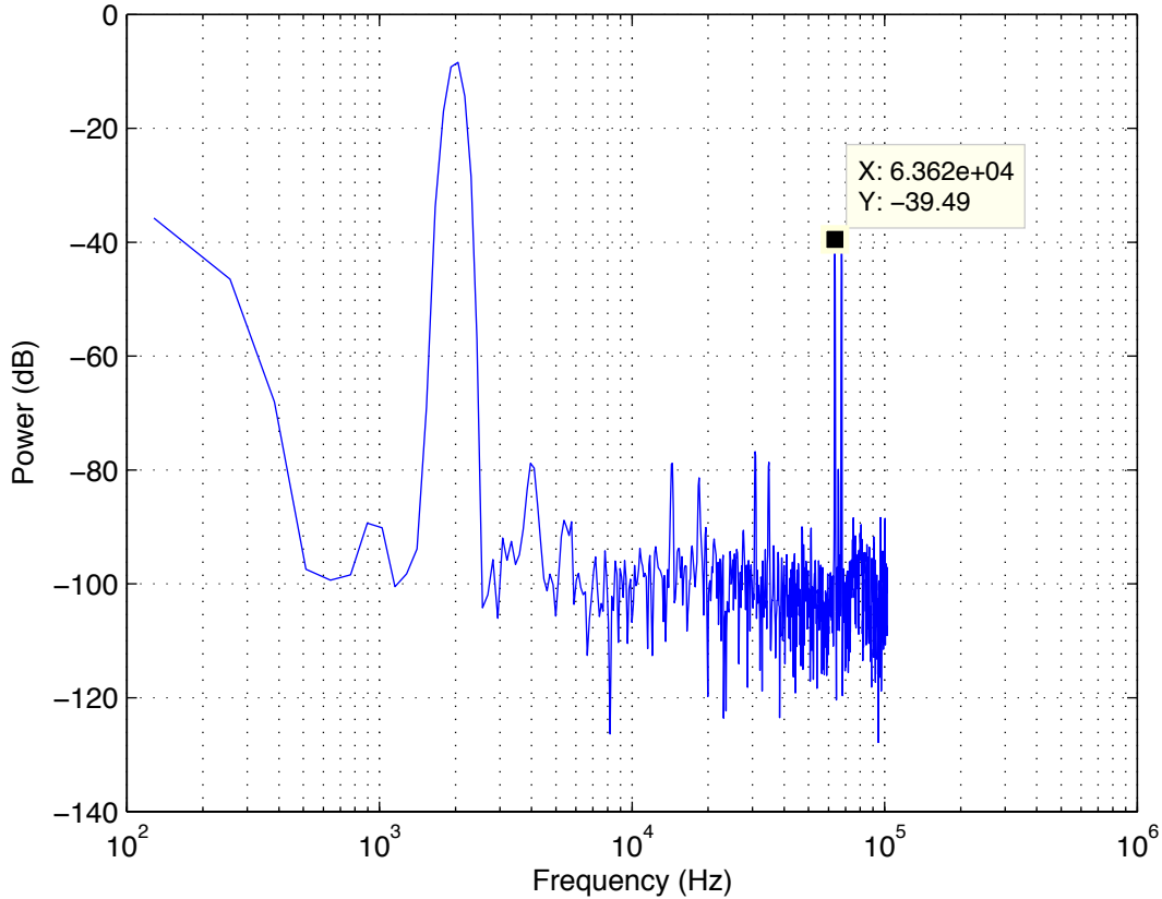
Power Spectrum of DAC at 1Y4 with 2kHz, 1000 counts amplitude sine wave from the DAC
