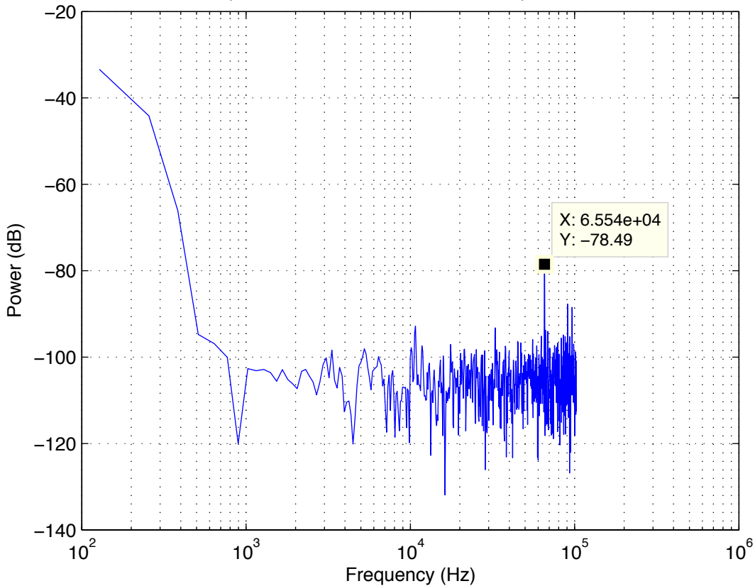
Power Spectrum of DAC at 1Y4 with no output from the DAC
