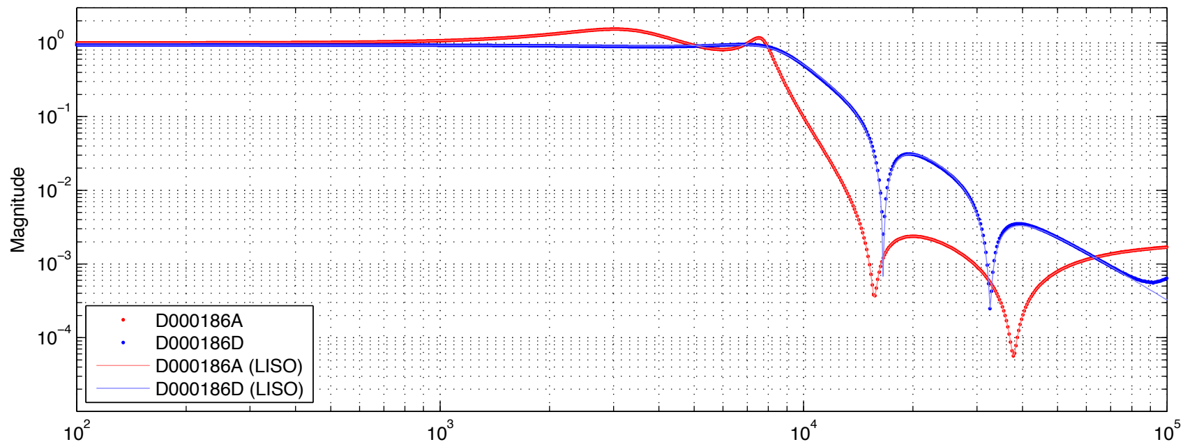
D000186A/D Transfer function (2013/5/15)
