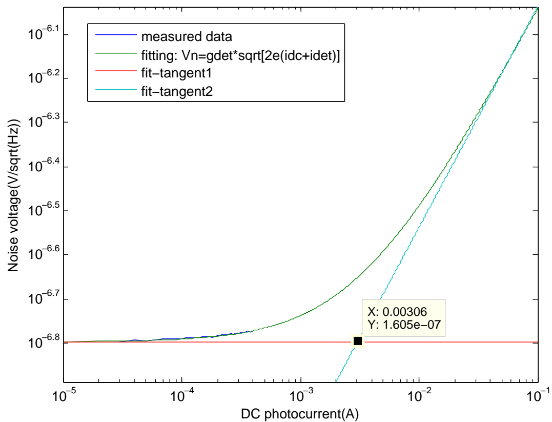
Noise level for PDA255
