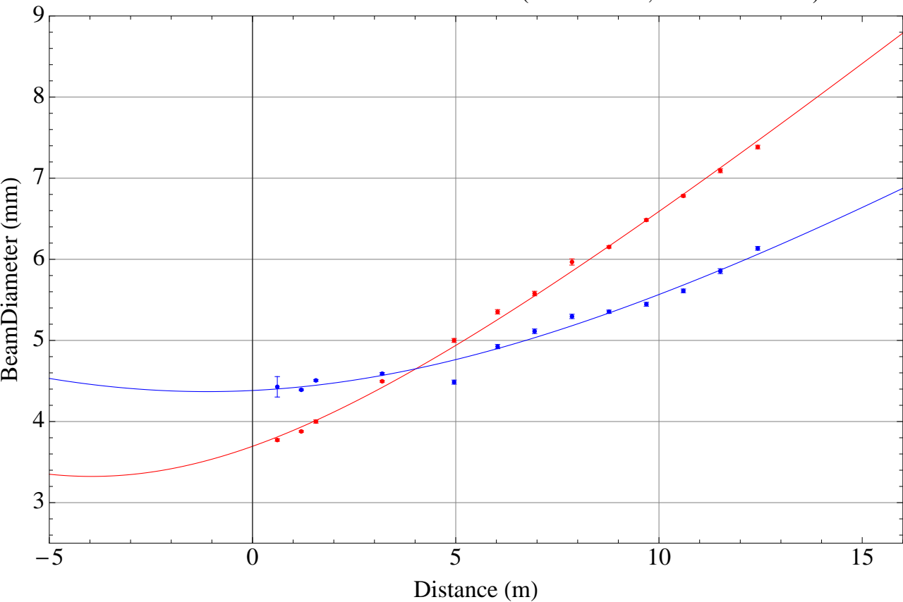
Beam Profile of the ITM Beam Reflection (Red=vertical, Blue=Horizontal)
