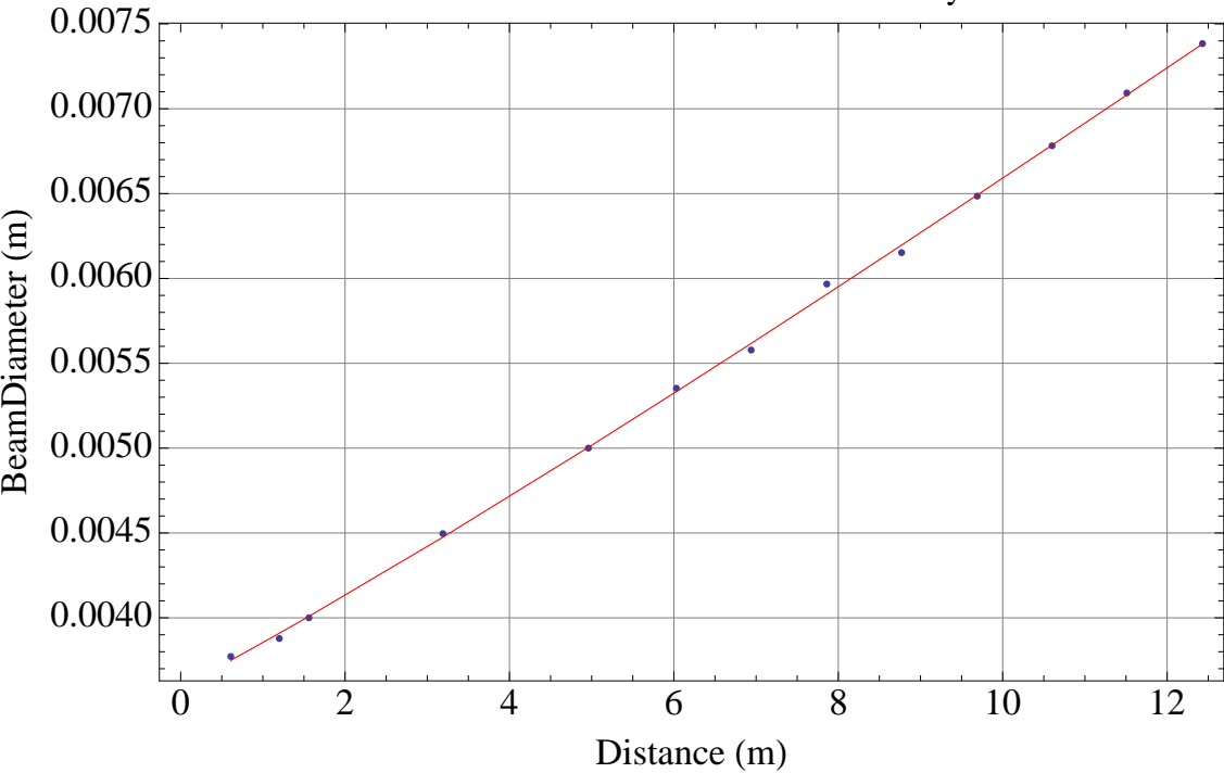
REFL Beam Profile of the beam reflected by PRM
