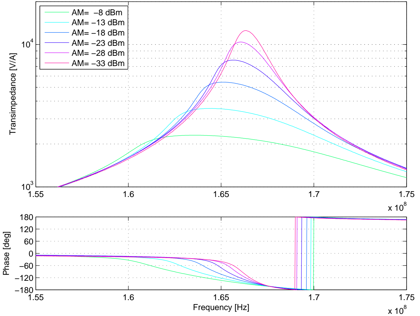
Effect of RF power level on REFL165 TF (2011/06/03)
