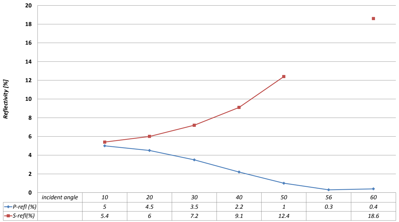
Reflectivity of green#14 welding glass
