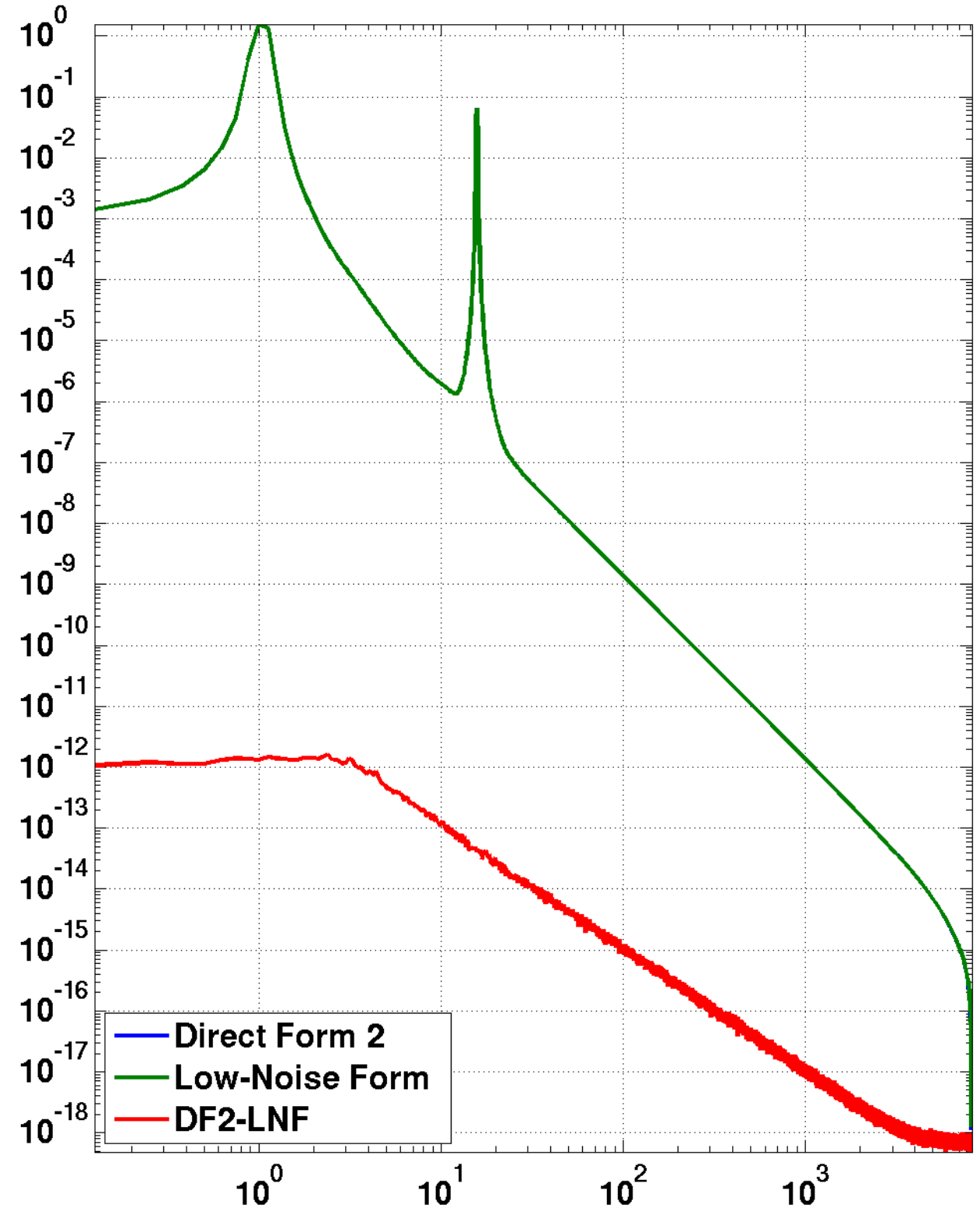
Double Precision
