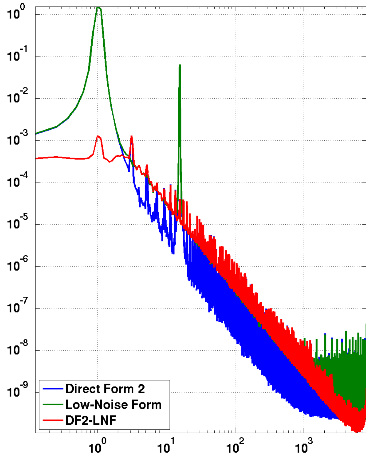
Single Precision
