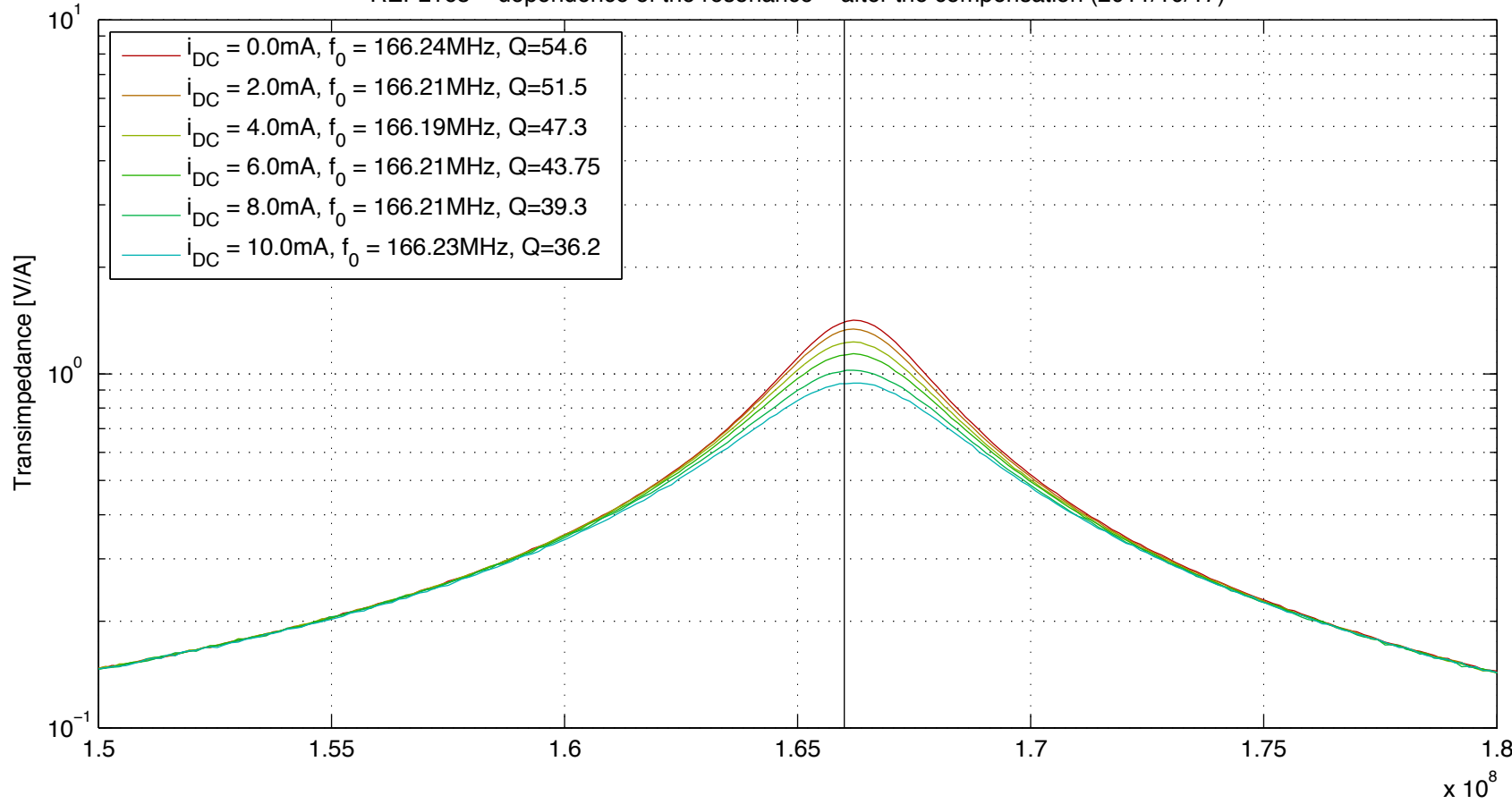
REFL165 – dependence of the resonance ~ after the compensation (2011/10/17)
