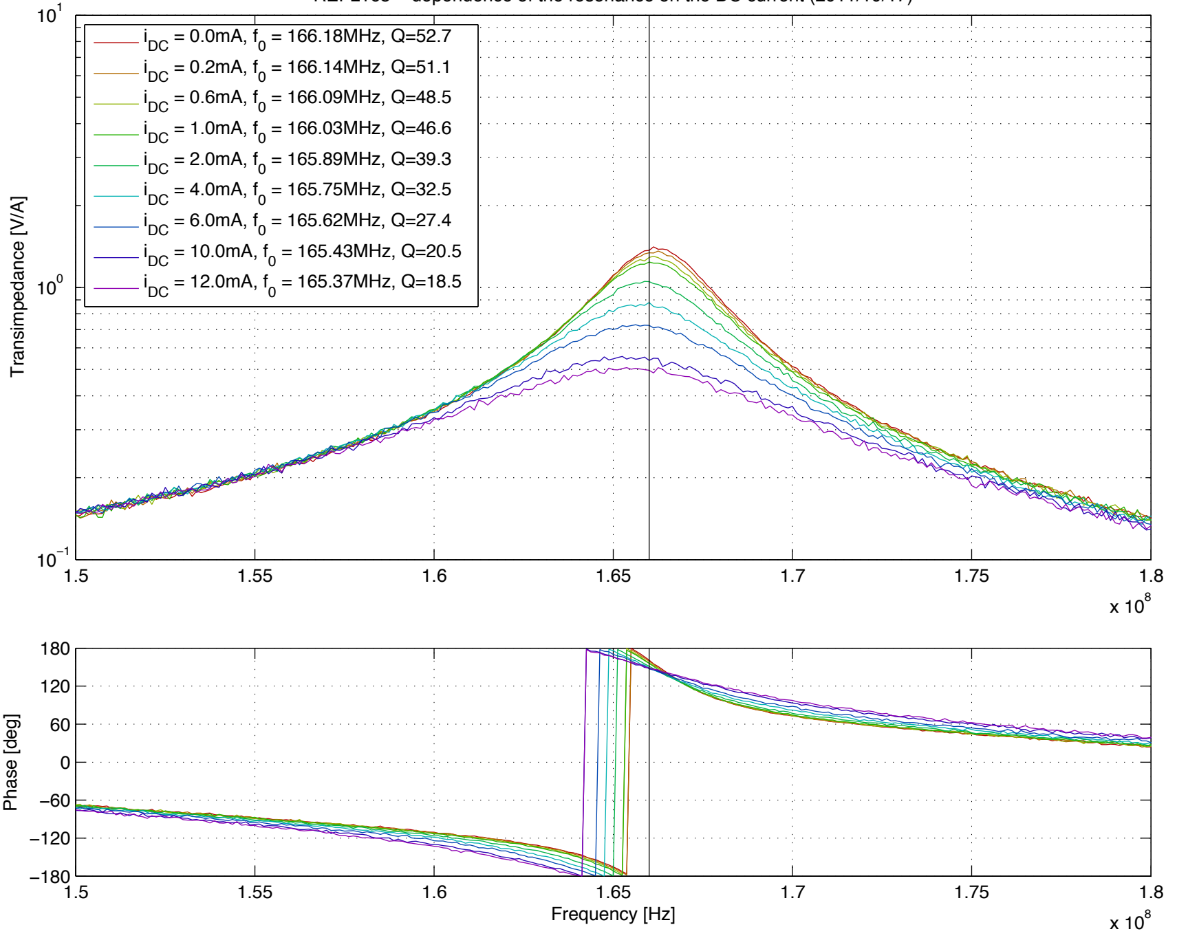
REFL165 – dependence of the resonance on the DC current (2011/10/17)
