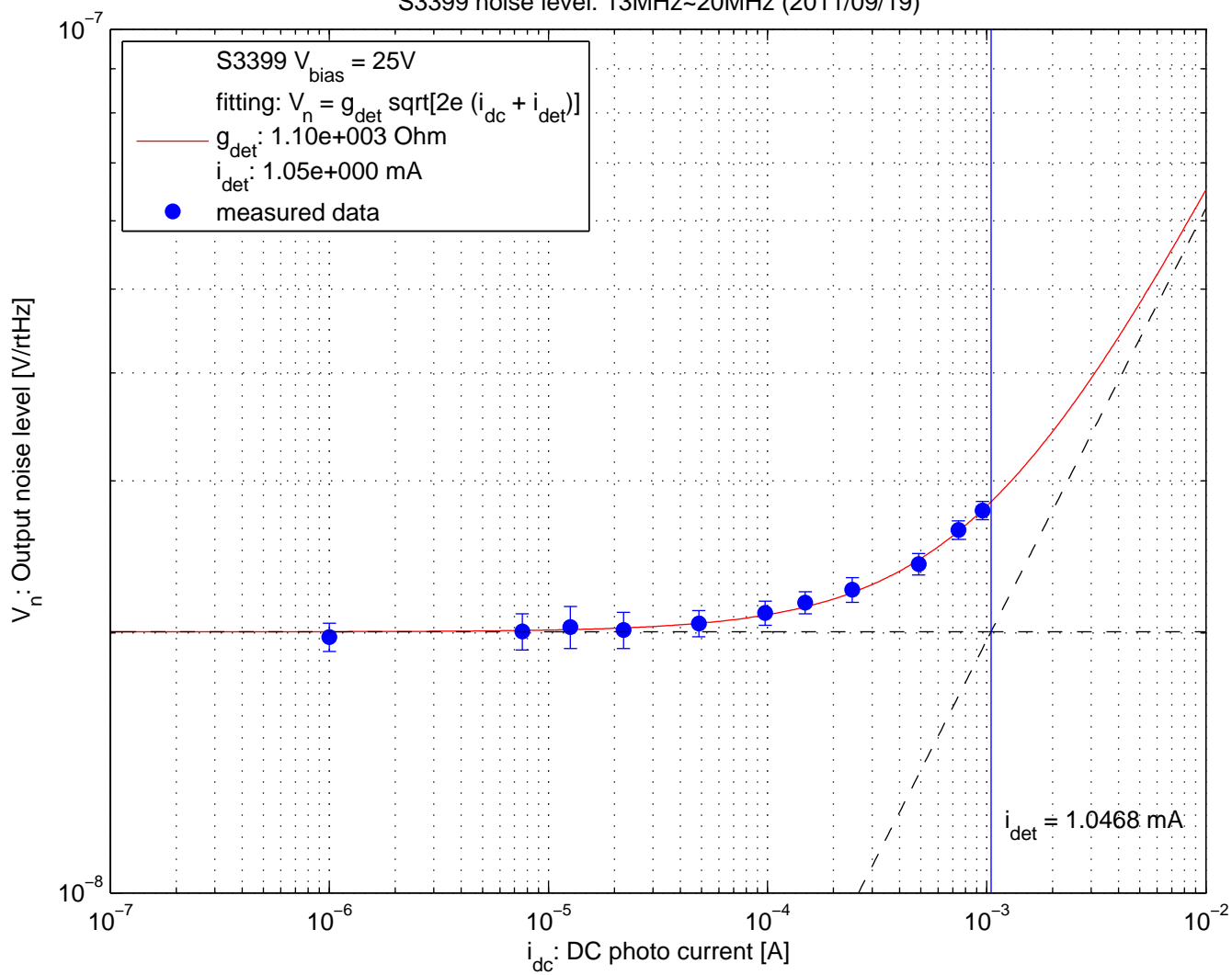
S3399 noise level: 13MHz~20MHz (2011/09/19)
