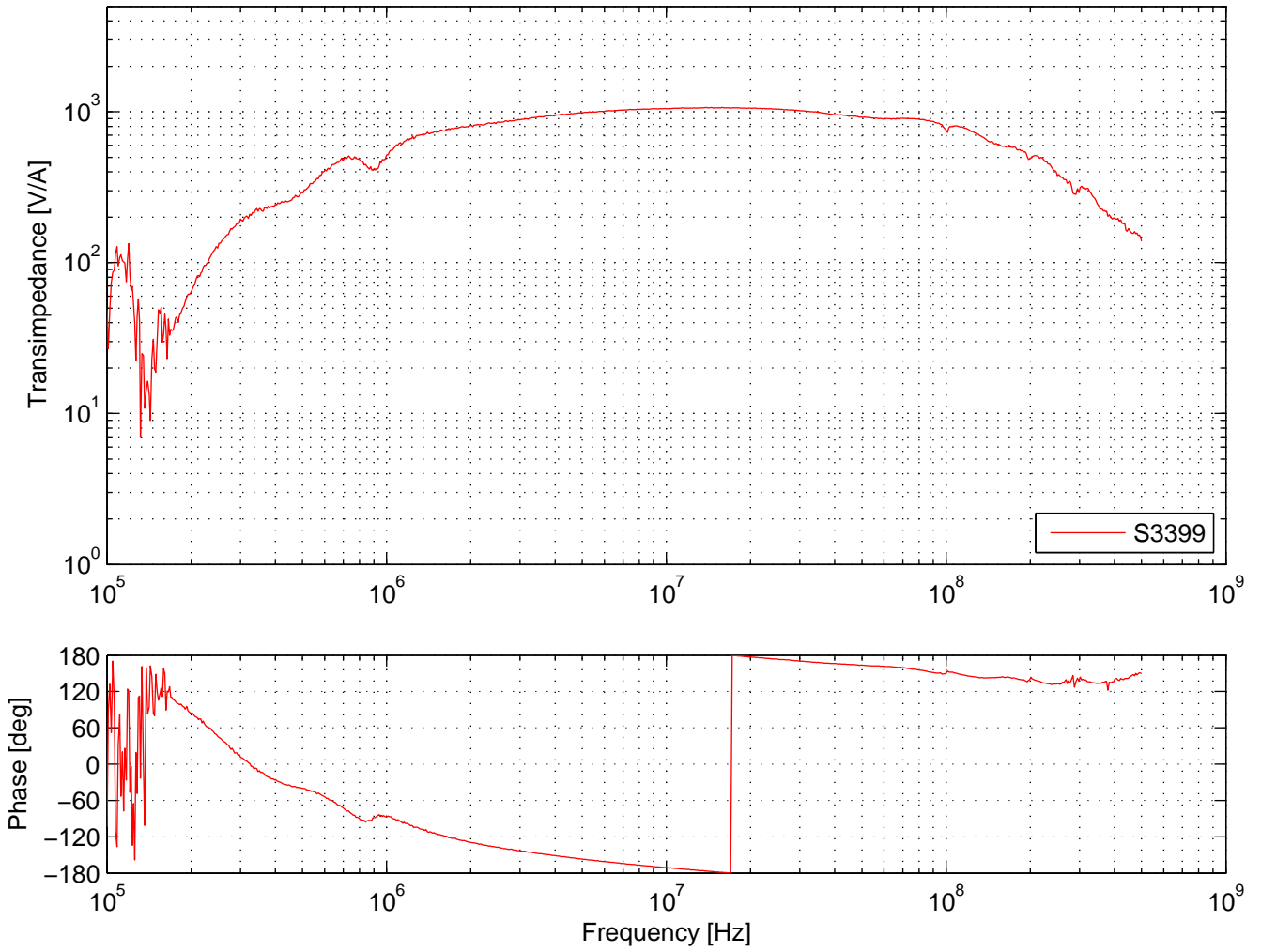
S3399 25V bias (2011/09/19)
