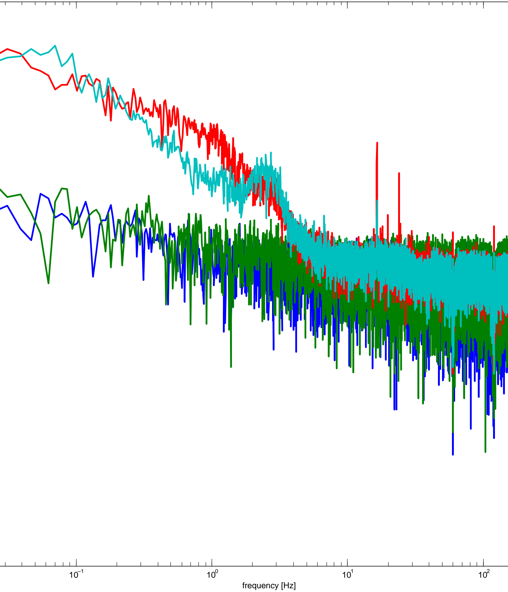
SRM QPD dark noise PSD (uncalibrated in angle)
