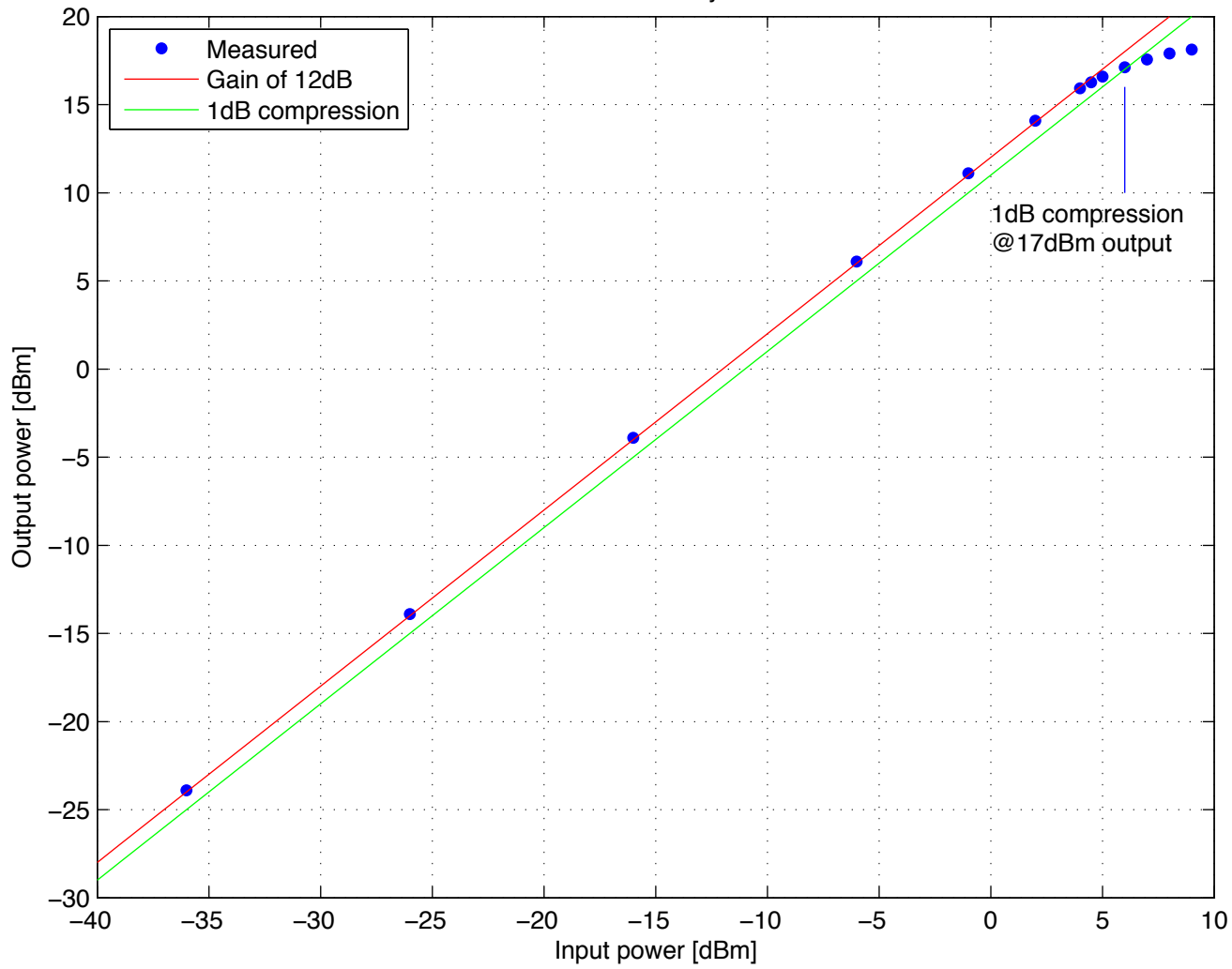
GALI-6 linearity test
