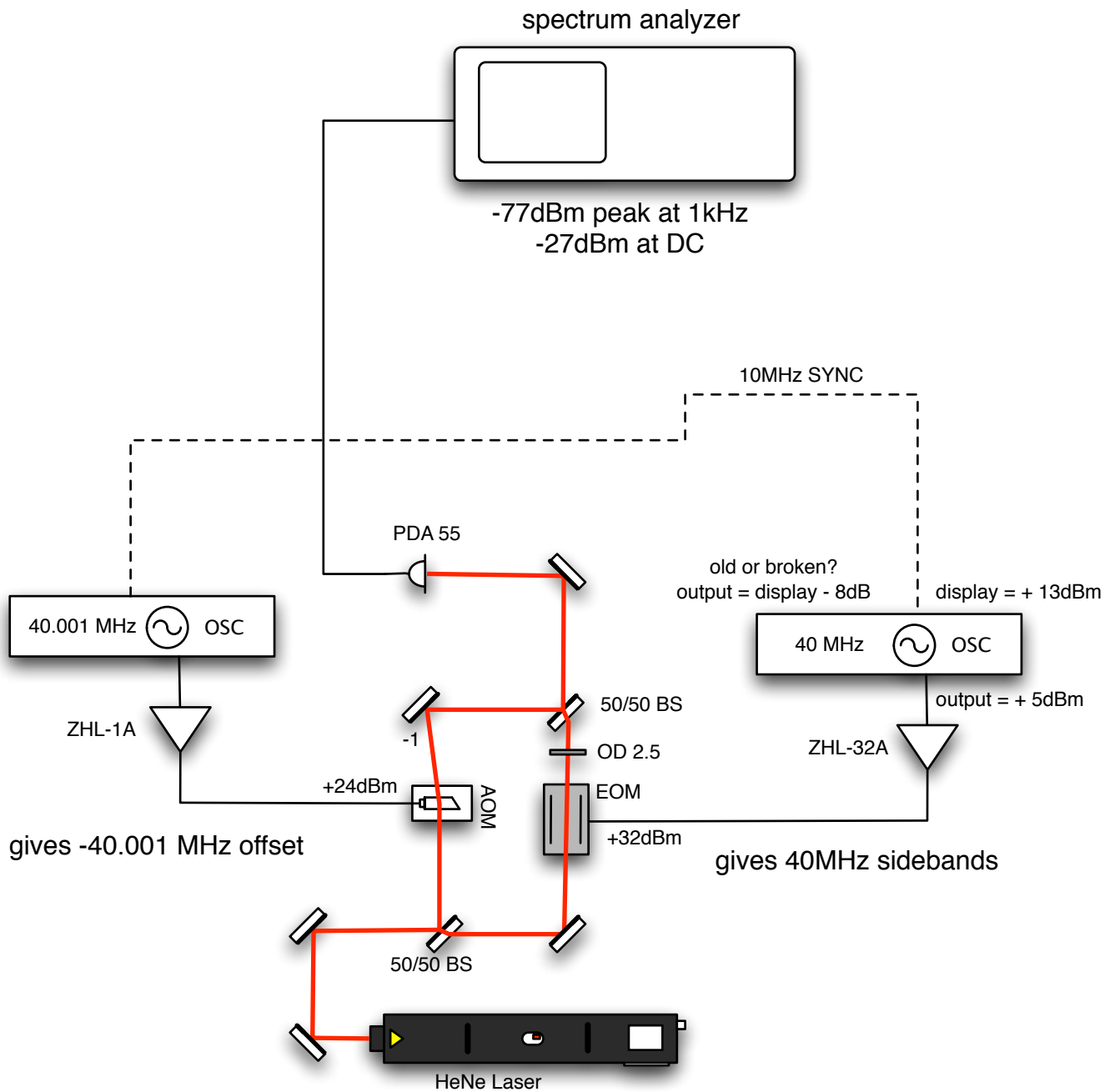
Phase camera layout - version 1 Summer 2010 (22nd June)
