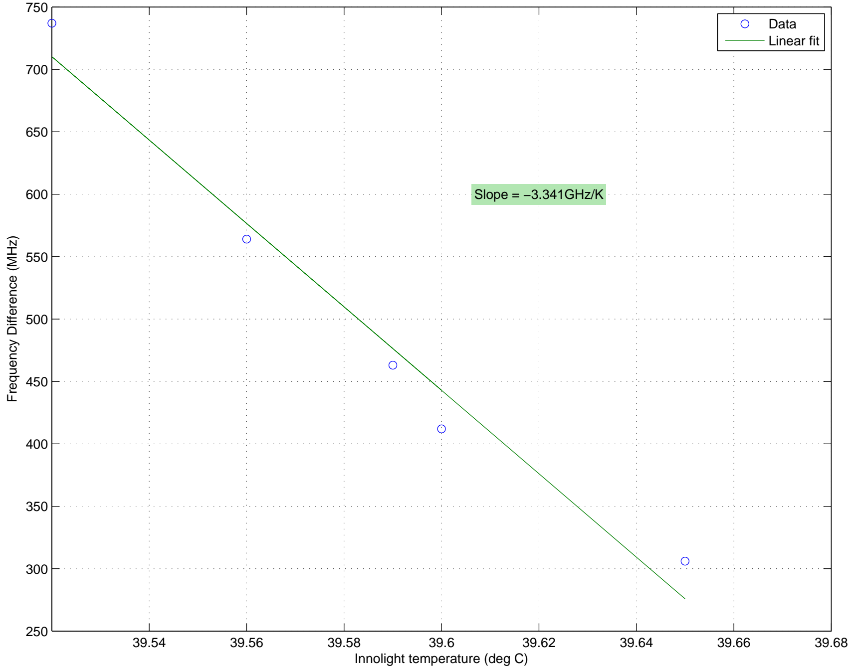
Innolight – Lightwave frequency difference versus Innolight temperature. LW temp = 37.2602 C
