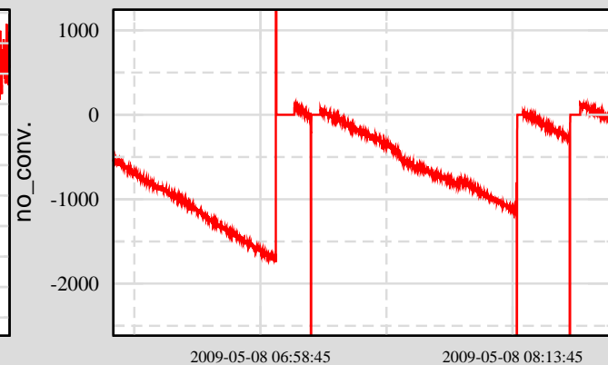
Ch 7: C1:LSC-DARM_OUT16
