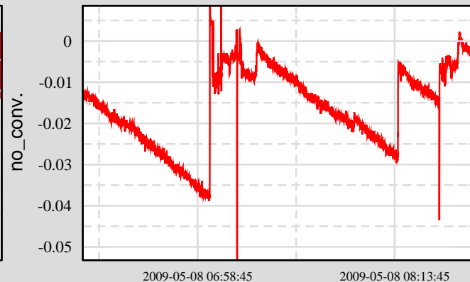
Ch 5: C1:SUS-ETMY_OPLEV_PERROR
