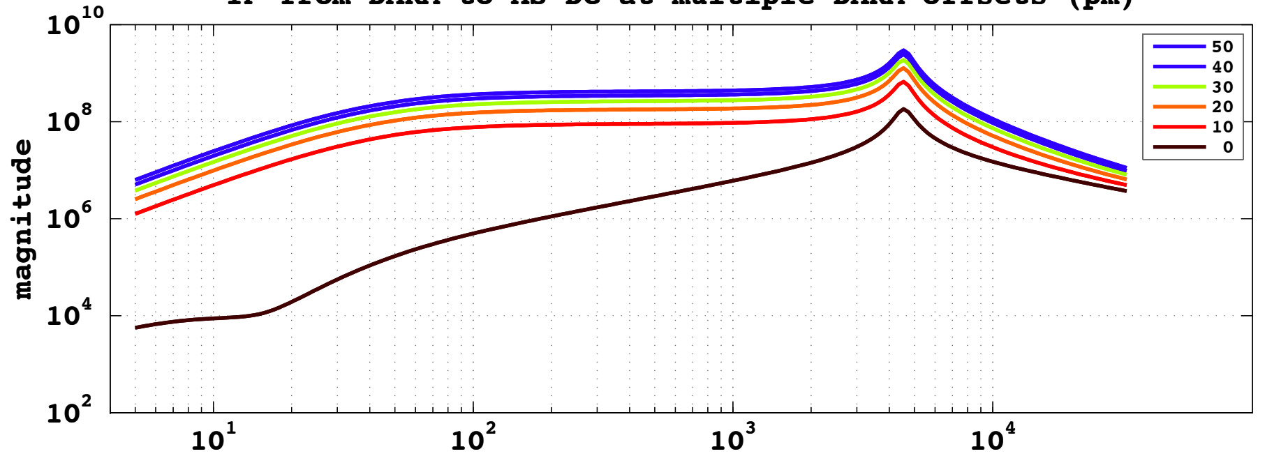
TF from DARM to AS DC at multiple DARM offsets (pm)
