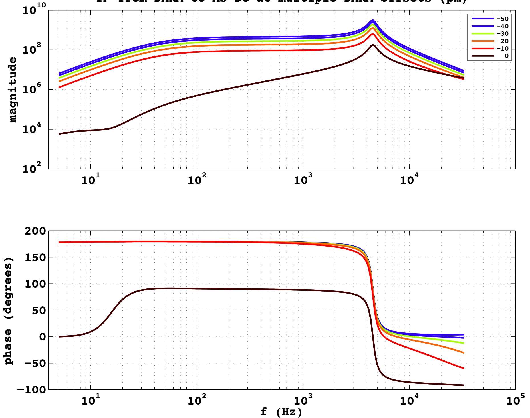
TF from DARM to AS DC at multiple DARM offsets (pm)
