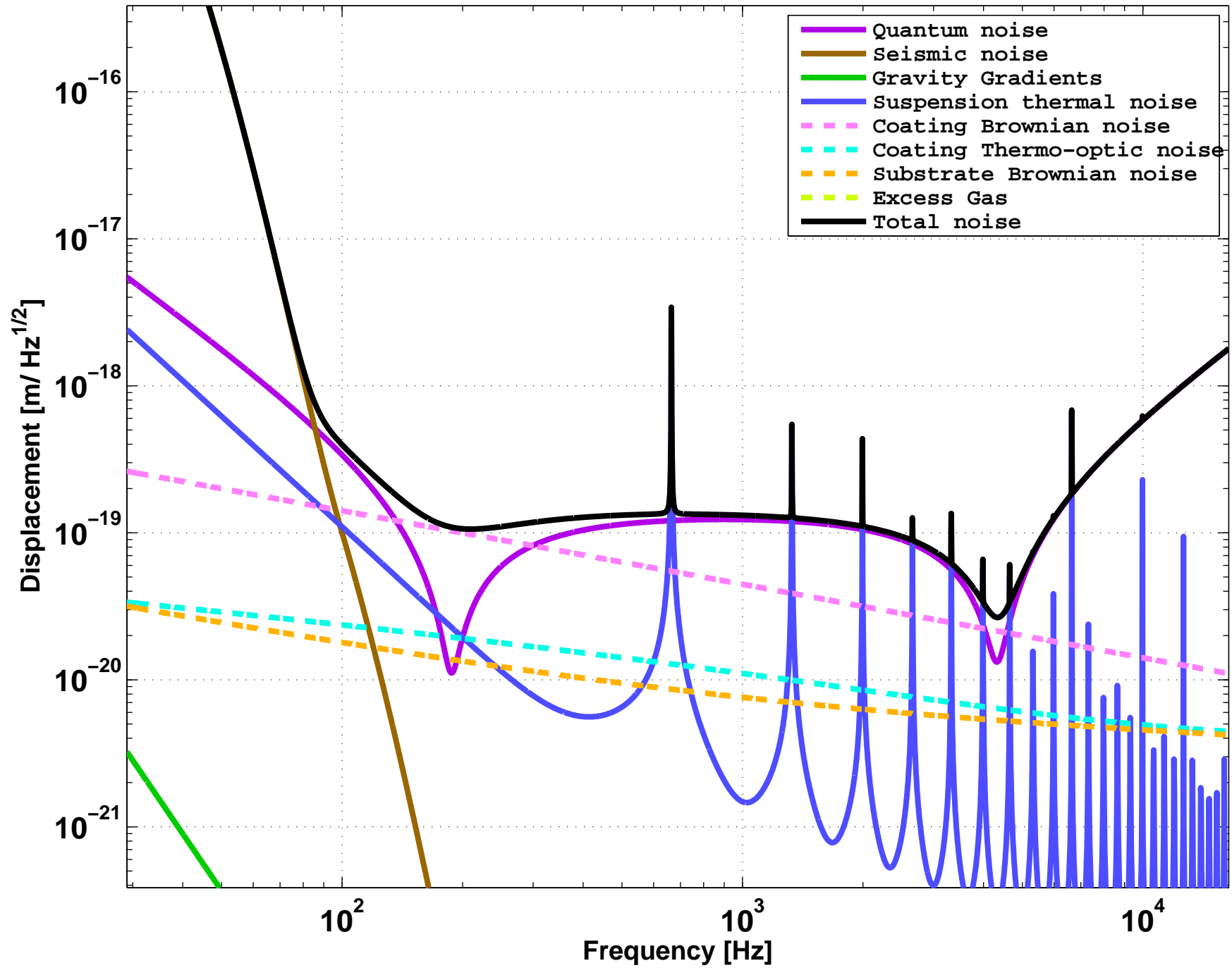
40m Displacement Noise w/ MOSs (P = 3 W)
