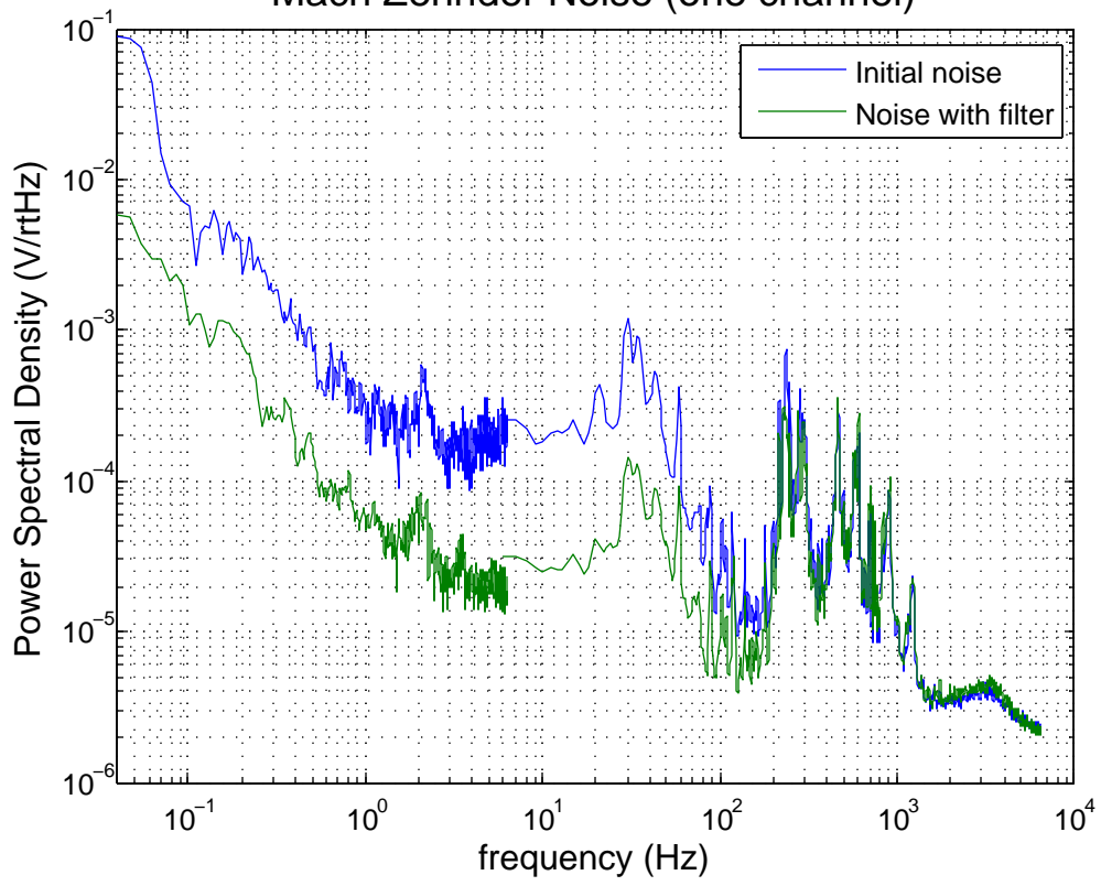
Mach Zehnder Noise (one channel)
